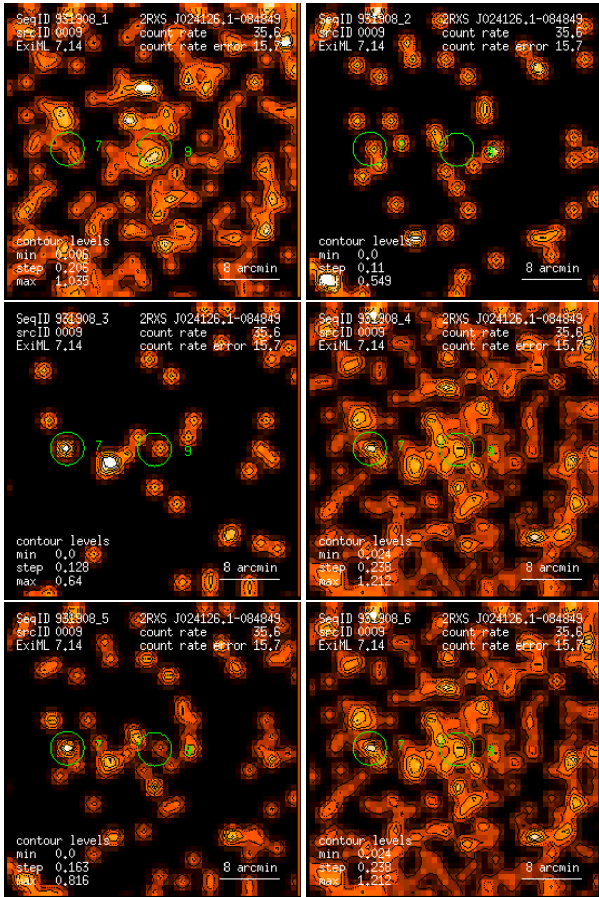
Figure 9: RASS 931908: detection 0009: band rate images, Gaussian filter: (1) PSPC channels 11 – 41, (2) 52 – 90, (3) 91 – 201, (4) 11 – 235, (5) 52 – 201, (6) 11 – 201. Broad band rates in counts/ks. Band rate contour levels in counts/ks/arcmin 2 .
