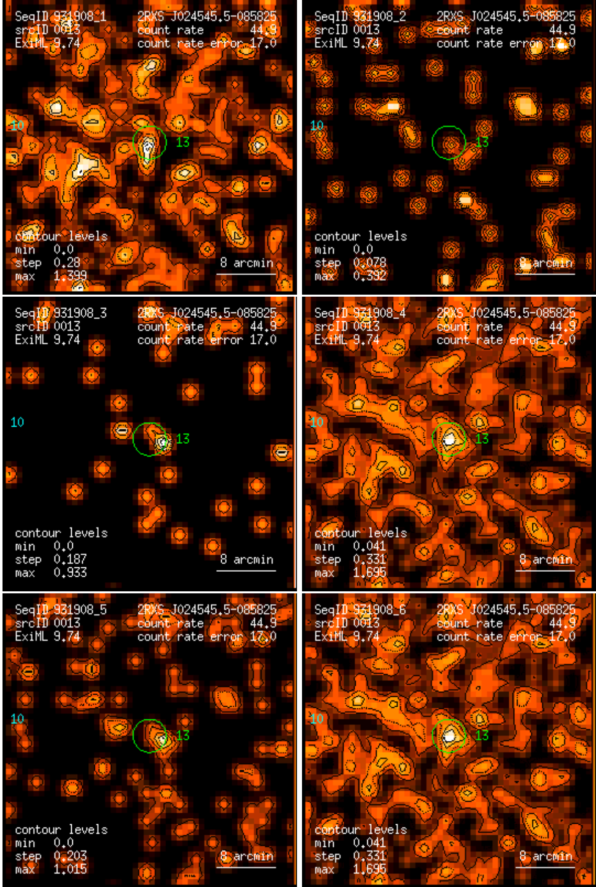
Figure 13: RASS 931908: detection 0013: band rate images, Gaussian filter: (1) PSPC channels 11 – 41, (2) 52 – 90, (3) 91 – 201, (4) 11 – 235, (5) 52 – 201, (6) 11 – 201. Broad band rates in counts/ks. Band rate contour levels in counts/ks/arcmin 2 .
