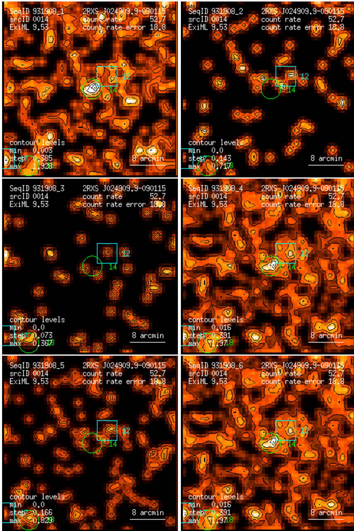
Figure 14: RASS 931908: detection 0014: band rate images, Gaussian filter: (1) PSPC channels 11 – 41, (2) 52 – 90, (3) 91 – 201, (4) 11 – 235, (5) 52 – 201, (6) 11 – 201. Broad band rates in counts/ks. Band rate contour levels in counts/ks/arcmin 2 .
