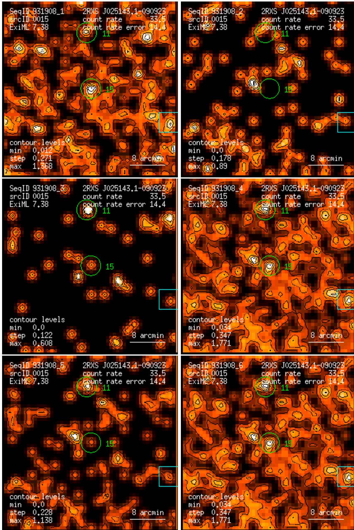
Figure 15: RASS 931908: detection 0015: band rate images, Gaussian filter: (1) PSPC channels 11 – 41, (2) 52 – 90, (3) 91 – 201, (4) 11 – 235, (5) 52 – 201, (6) 11 – 201. Broad band rates in counts/ks. Band rate contour levels in counts/ks/arcmin 2 .
