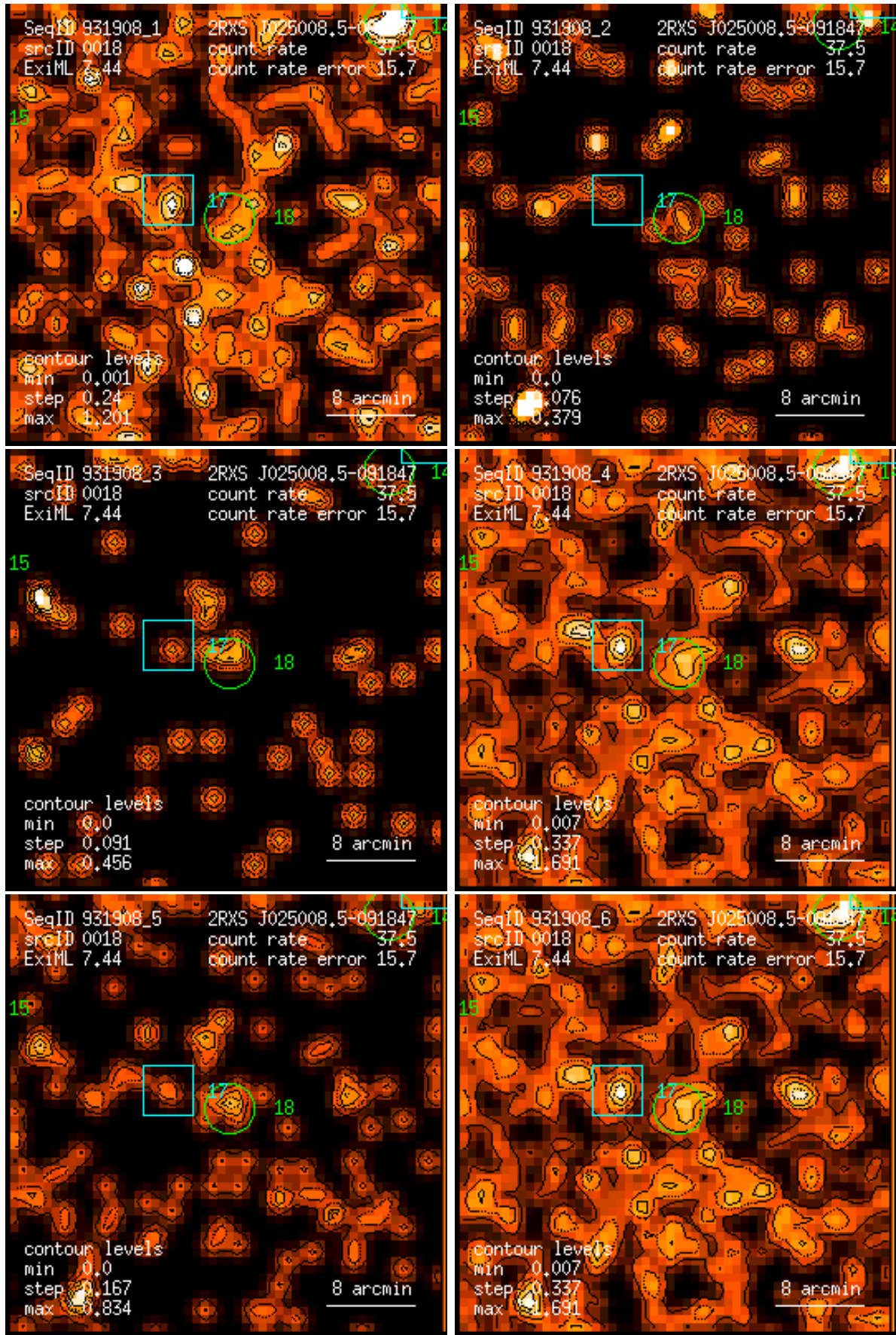
Figure 18: RASS 931908: detection 0018: band rate images, Gaussian filter: (1) PSPC channels 11 – 41, (2) 52 – 90, (3) 91 – 201, (4) 11 – 235, (5) 52 – 201, (6) 11 – 201. Broad band rates in counts/ks. Band rate contour levels in counts/ks/arcmin 2 .
