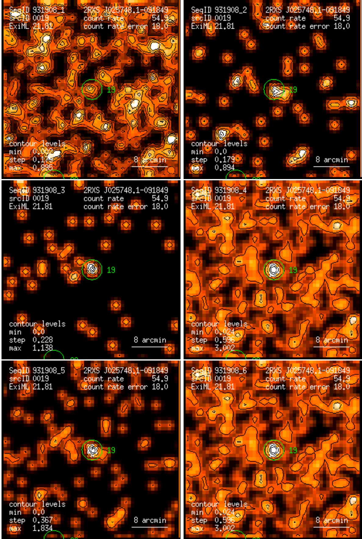
Figure 19: RASS 931908: detection 0019: band rate images, Gaussian filter: (1) PSPC channels 11 – 41, (2) 52 – 90, (3) 91 – 201, (4) 11 – 235, (5) 52 – 201, (6) 11 – 201. Broad band rates in counts/ks. Band rate contour levels in counts/ks/arcmin 2 .
