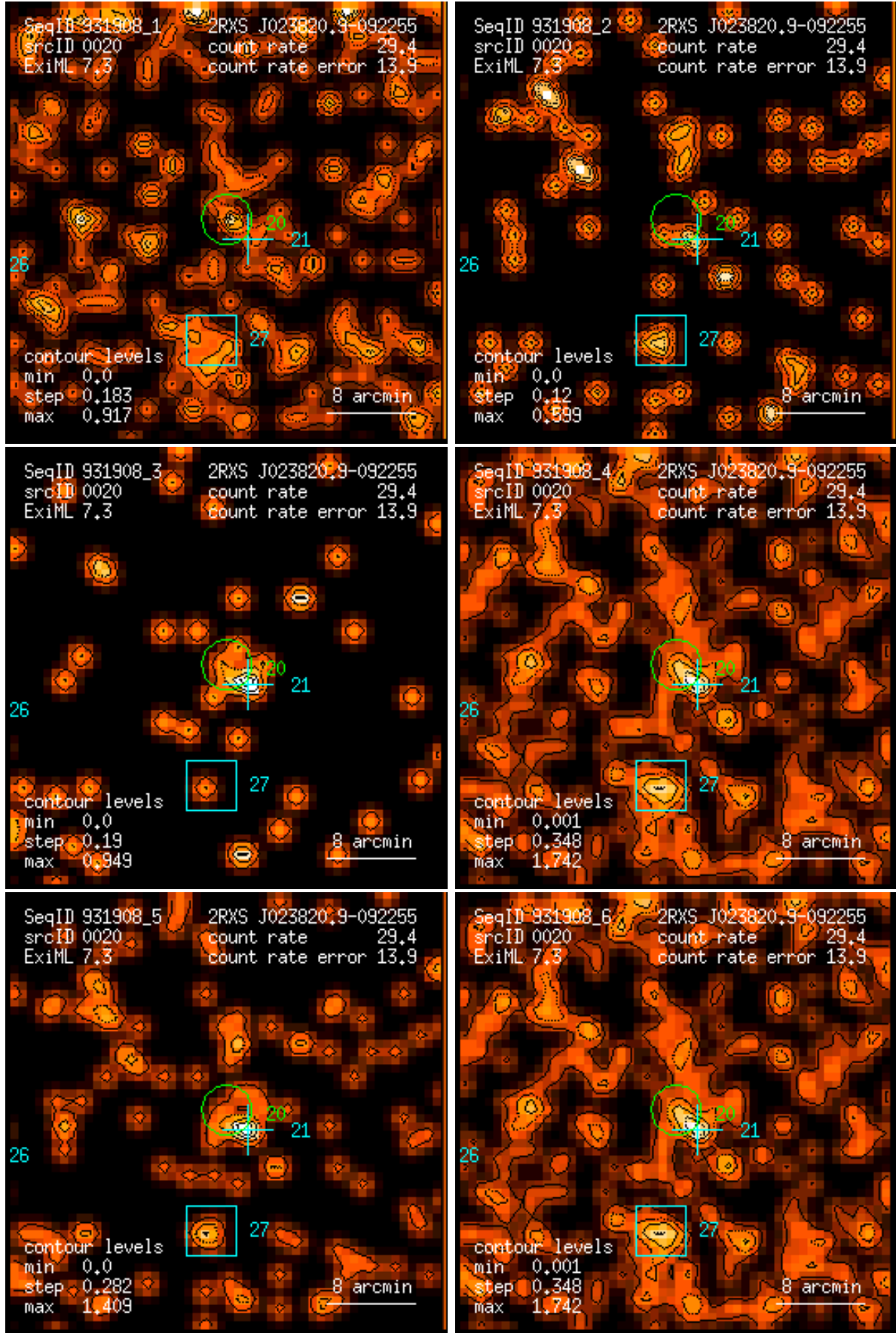
Figure 20: RASS 931908: detection 0020: band rate images, Gaussian filter: (1) PSPC channels 11 – 41, (2) 52 – 90, (3) 91 – 201, (4) 11 – 235, (5) 52 – 201, (6) 11 – 201. Broad band rates in counts/ks. Band rate contour levels in counts/ks/arcmin 2 .
