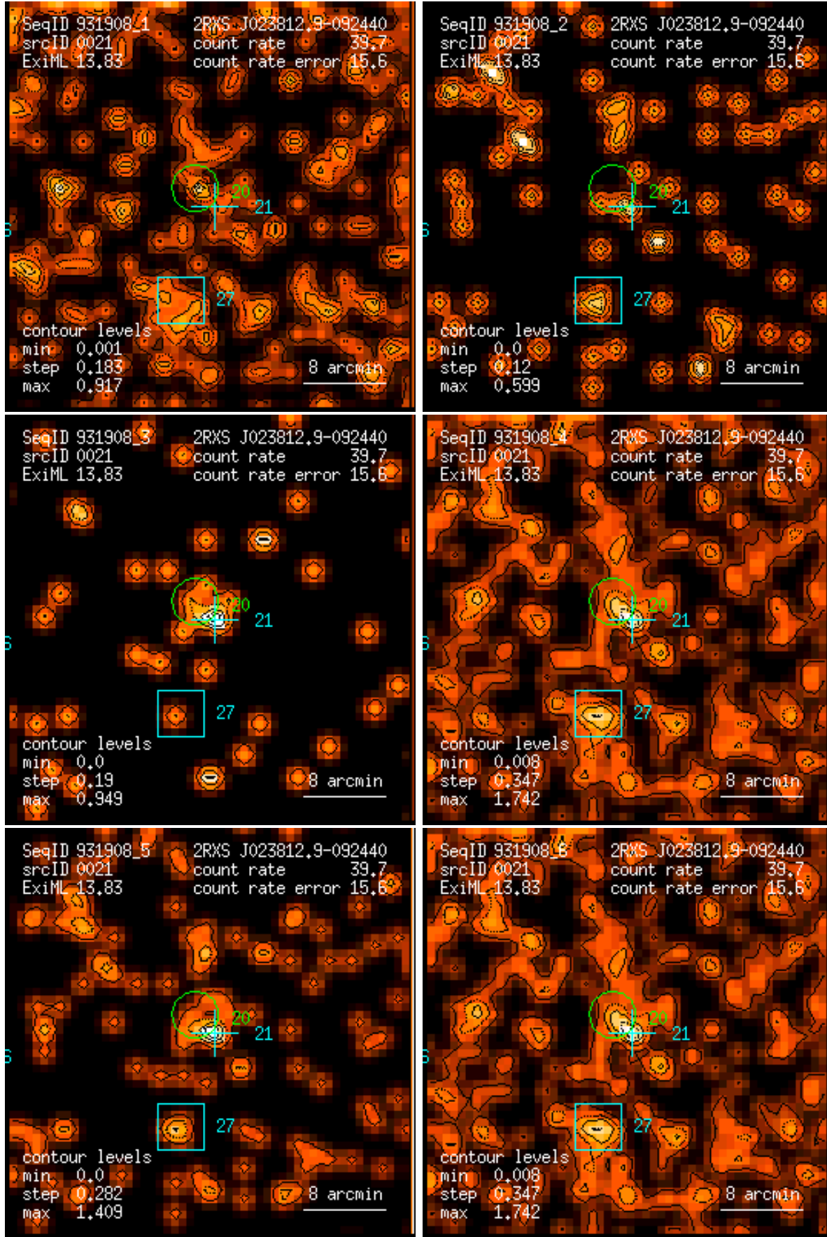
Figure 21: RASS 931908: detection 0021: band rate images, Gaussian filter: (1) PSPC channels 11 – 41, (2) 52 – 90, (3) 91 – 201, (4) 11 – 235, (5) 52 – 201, (6) 11 – 201. Broad band rates in counts/ks. Band rate contour levels in counts/ks/arcmin 2 .
