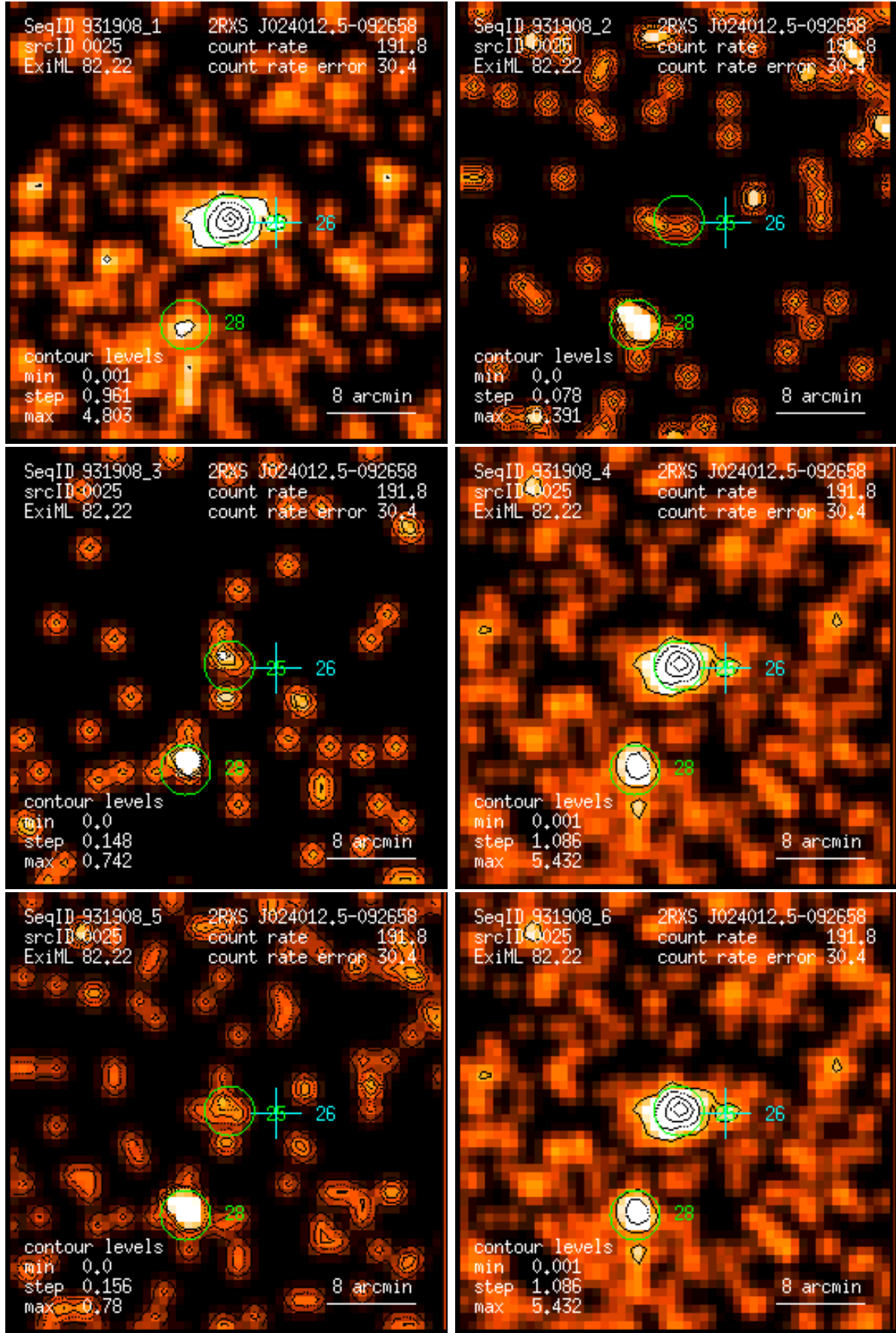
Figure 25: RASS 931908: detection 0025: band rate images, Gaussian filter: (1) PSPC channels 11 – 41, (2) 52 – 90, (3) 91 – 201, (4) 11 – 235, (5) 52 – 201, (6) 11 – 201. Broad band rates in counts/ks. Band rate contour levels in counts/ks/arcmin 2 .
