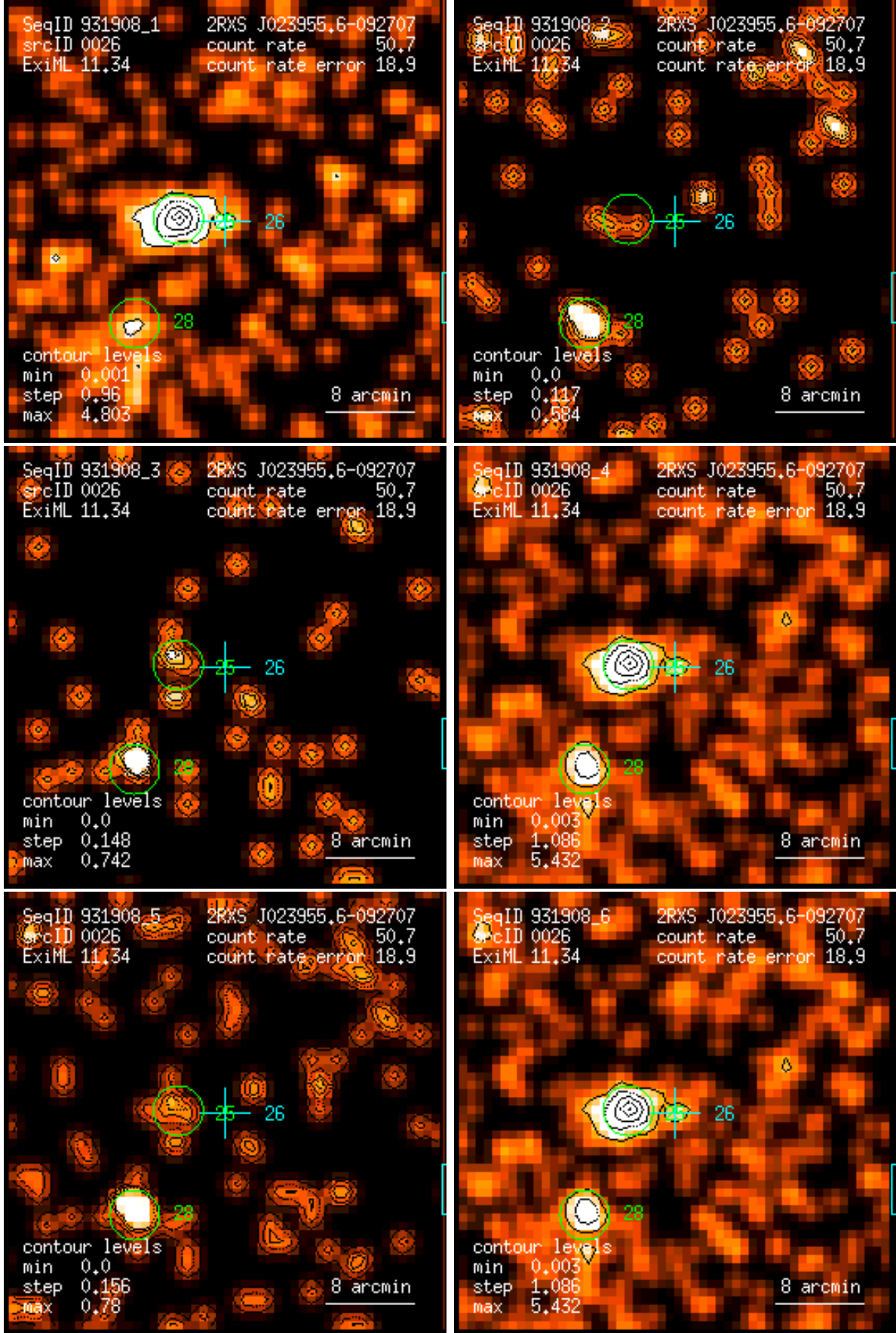
Figure 26: RASS 931908: detection 0026: band rate images, Gaussian filter: (1) PSPC channels 11 – 41, (2) 52 – 90, (3) 91 – 201, (4) 11 – 235, (5) 52 – 201, (6) 11 – 201. Broad band rates in counts/ks. Band rate contour levels in counts/ks/arcmin 2 .
