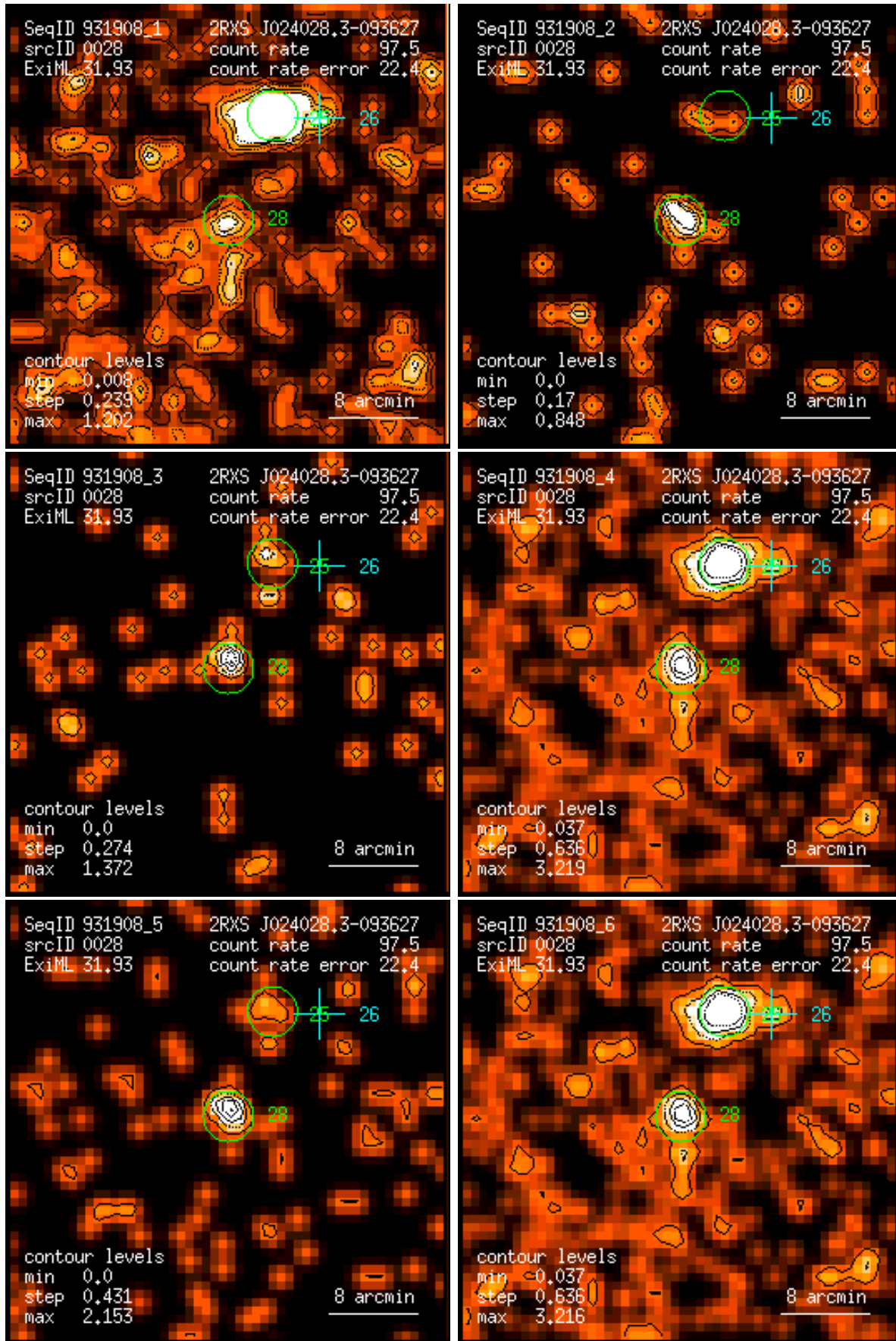
Figure 28: RASS 931908: detection 0028: band rate images, Gaussian filter: (1) PSPC channels 11 – 41, (2) 52 – 90, (3) 91 – 201, (4) 11 – 235, (5) 52 – 201, (6) 11 – 201. Broad band rates in counts/ks. Band rate contour levels in counts/ks/arcmin 2 .
