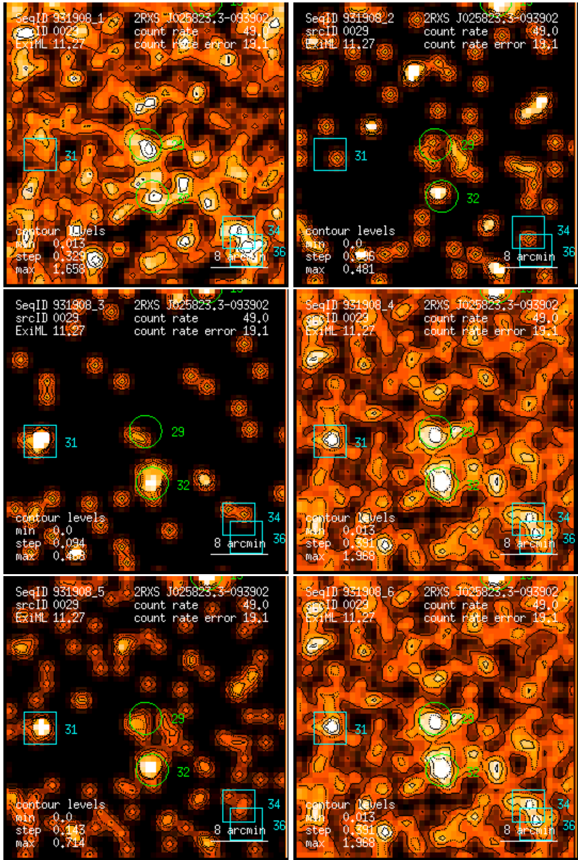
Figure 29: RASS 931908: detection 0029: band rate images, Gaussian filter: (1) PSPC channels 11 – 41, (2) 52 – 90, (3) 91 – 201, (4) 11 – 235, (5) 52 – 201, (6) 11 – 201. Broad band rates in counts/ks. Band rate contour levels in counts/ks/arcmin 2 .
