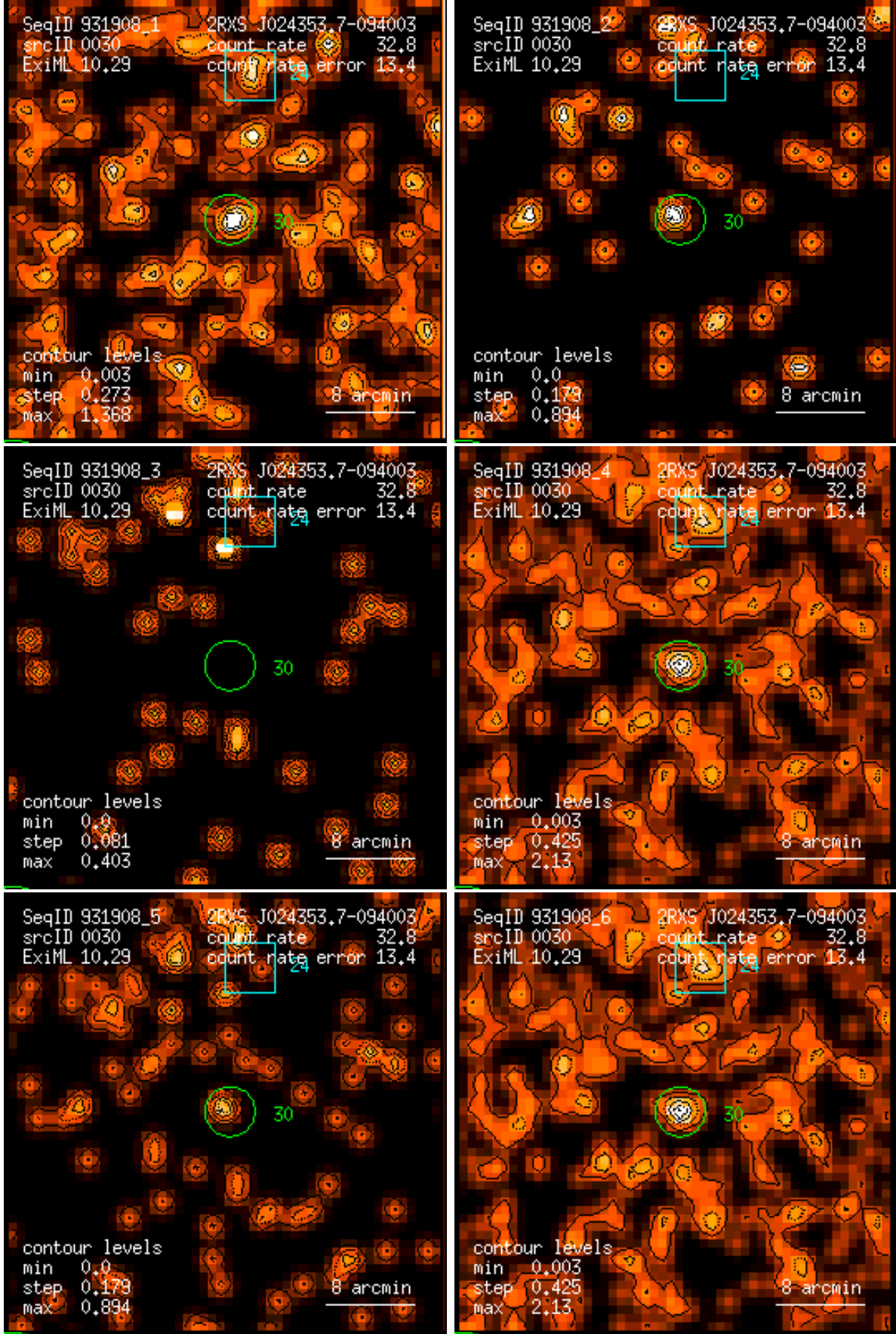
Figure 30: RASS 931908: detection 0030: band rate images, Gaussian filter: (1) PSPC channels 11 – 41, (2) 52 – 90, (3) 91 – 201, (4) 11 – 235, (5) 52 – 201, (6) 11 – 201. Broad band rates in counts/ks. Band rate contour levels in counts/ks/arcmin 2 .
