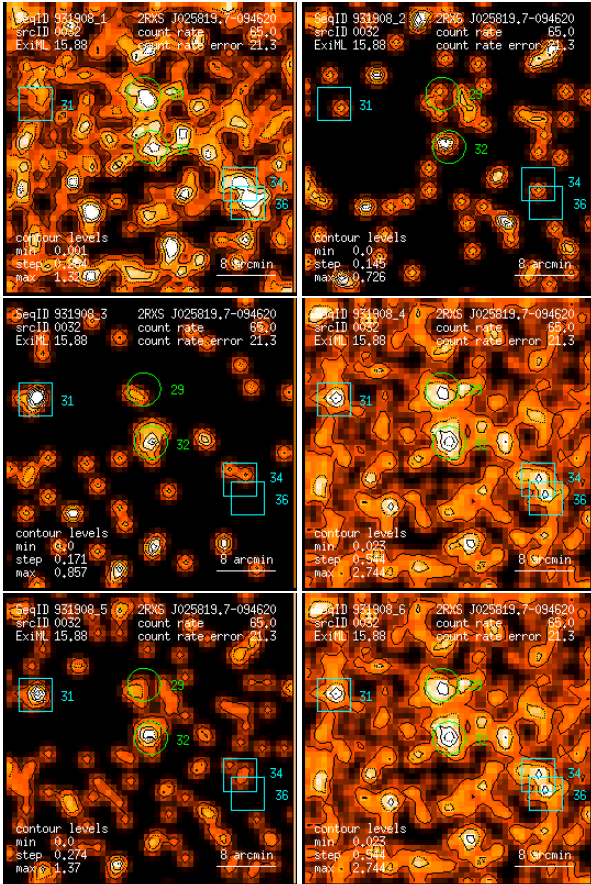
Figure 32: RASS 931908: detection 0032: band rate images, Gaussian filter: (1) PSPC channels 11 – 41, (2) 52 – 90, (3) 91 – 201, (4) 11 – 235, (5) 52 – 201, (6) 11 – 201. Broad band rates in counts/ks. Band rate contour levels in counts/ks/arcmin 2 .
