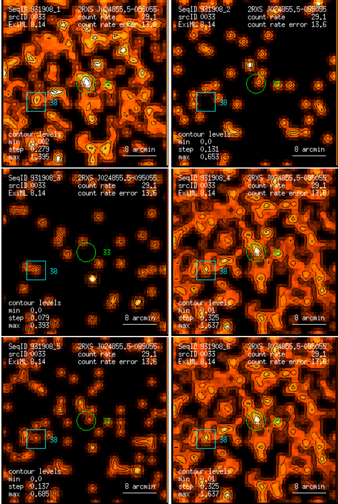
Figure 33: RASS 931908: detection 0033: band rate images, Gaussian filter: (1) PSPC channels 11 – 41, (2) 52 – 90, (3) 91 – 201, (4) 11 – 235, (5) 52 – 201, (6) 11 – 201. Broad band rates in counts/ks. Band rate contour levels in counts/ks/arcmin 2 .
