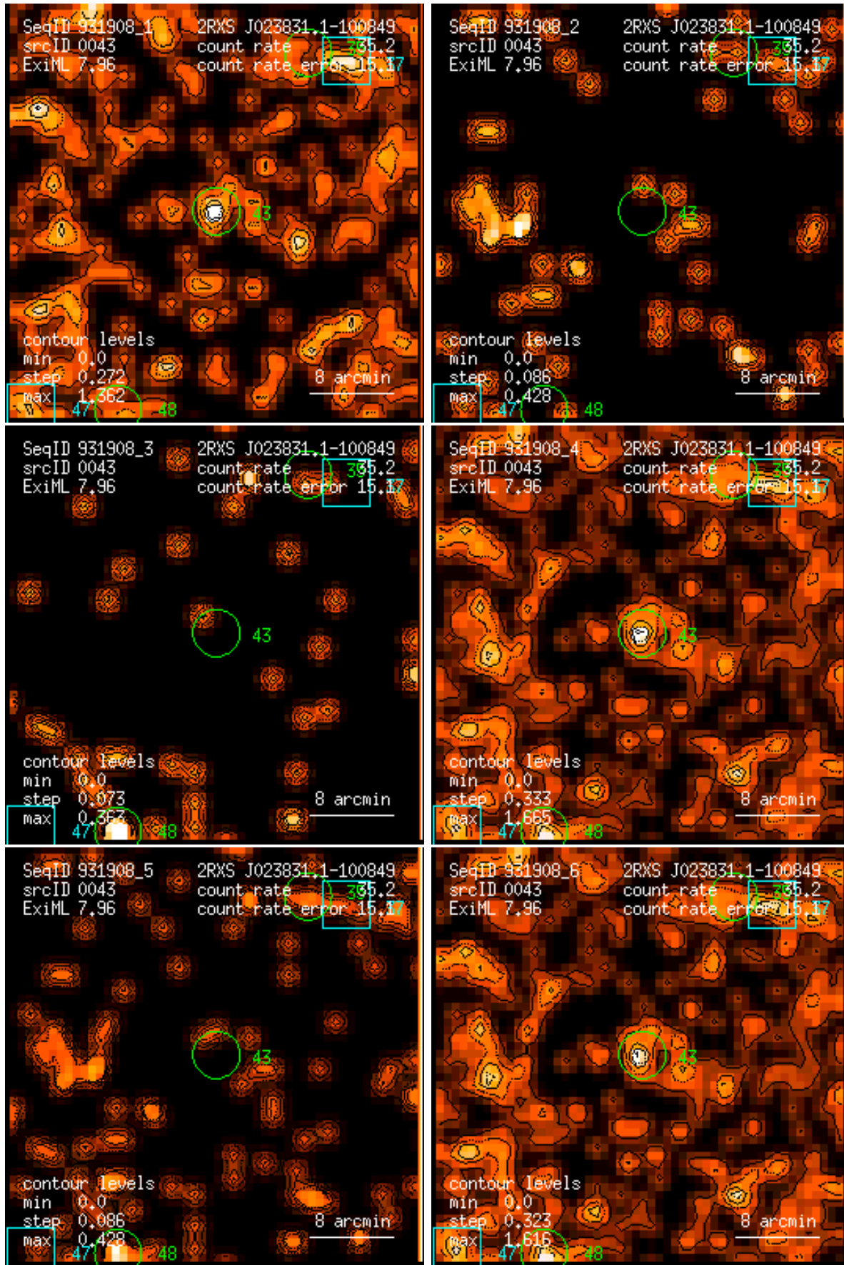
Figure 43: RASS 931908: detection 0043: band rate images, Gaussian filter: (1) PSPC channels 11 – 41, (2) 52 – 90, (3) 91 – 201, (4) 11 – 235, (5) 52 – 201, (6) 11 – 201. Broad band rates in counts/ks. Band rate contour levels in counts/ks/arcmin 2 .
