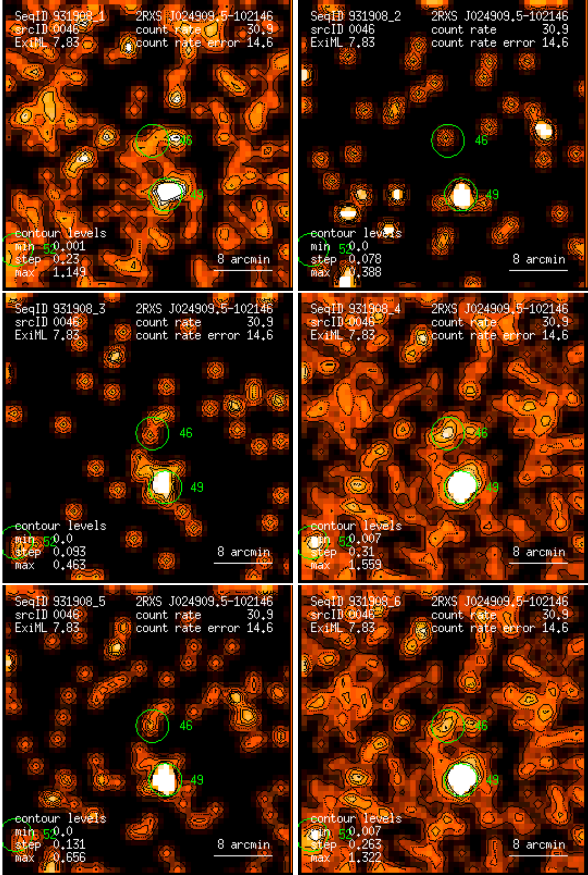
Figure 46: RASS 931908: detection 0046: band rate images, Gaussian filter: (1) PSPC channels 11 – 41, (2) 52 – 90, (3) 91 – 201, (4) 11 – 235, (5) 52 – 201, (6) 11 – 201. Broad band rates in counts/ks. Band rate contour levels in counts/ks/arcmin 2 .
