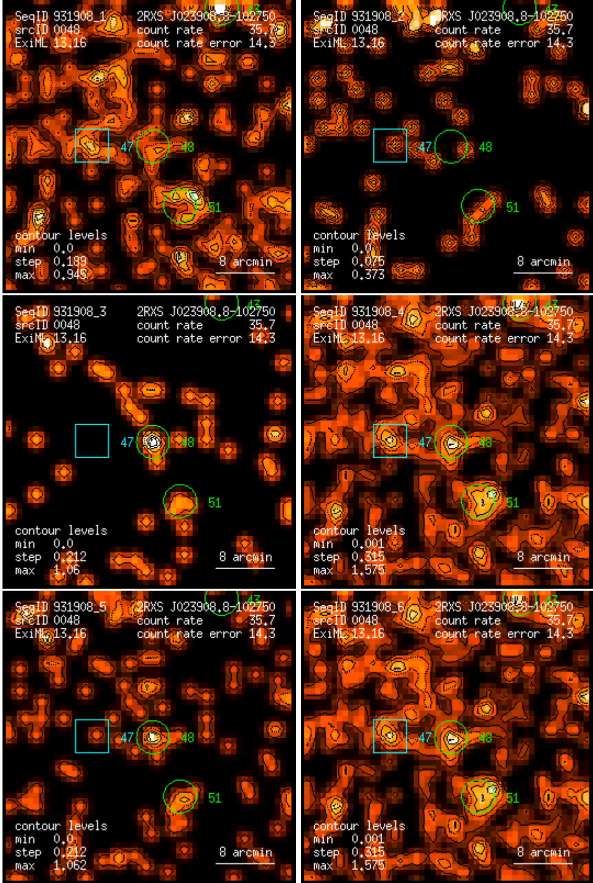
Figure 48: RASS 931908: detection 0048: band rate images, Gaussian filter: (1) PSPC channels 11 – 41, (2) 52 – 90, (3) 91 – 201, (4) 11 – 235, (5) 52 – 201, (6) 11 – 201. Broad band rates in counts/ks. Band rate contour levels in counts/ks/arcmin 2 .
