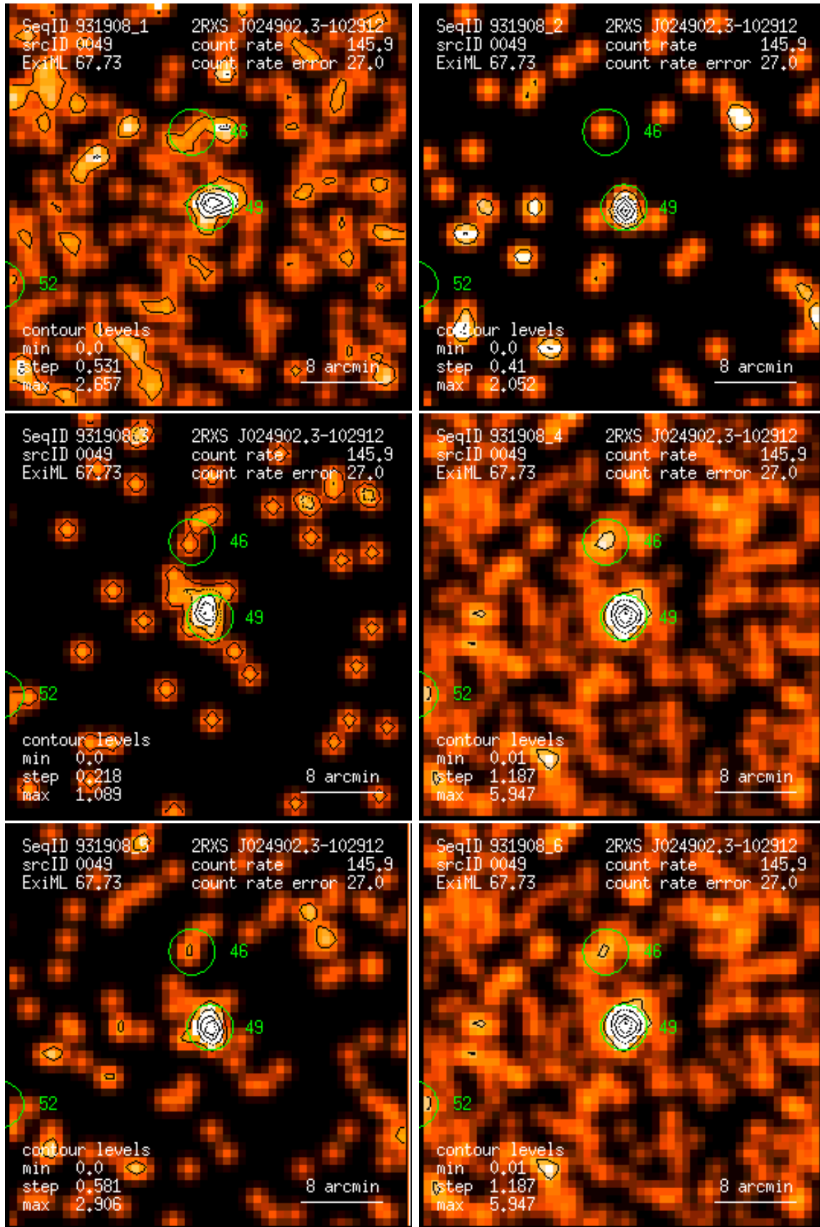
Figure 49: RASS 931908: detection 0049: band rate images, Gaussian filter: (1) PSPC channels 11 – 41, (2) 52 – 90, (3) 91 – 201, (4) 11 – 235, (5) 52 – 201, (6) 11 – 201. Broad band rates in counts/ks. Band rate contour levels in counts/ks/arcmin 2 .
