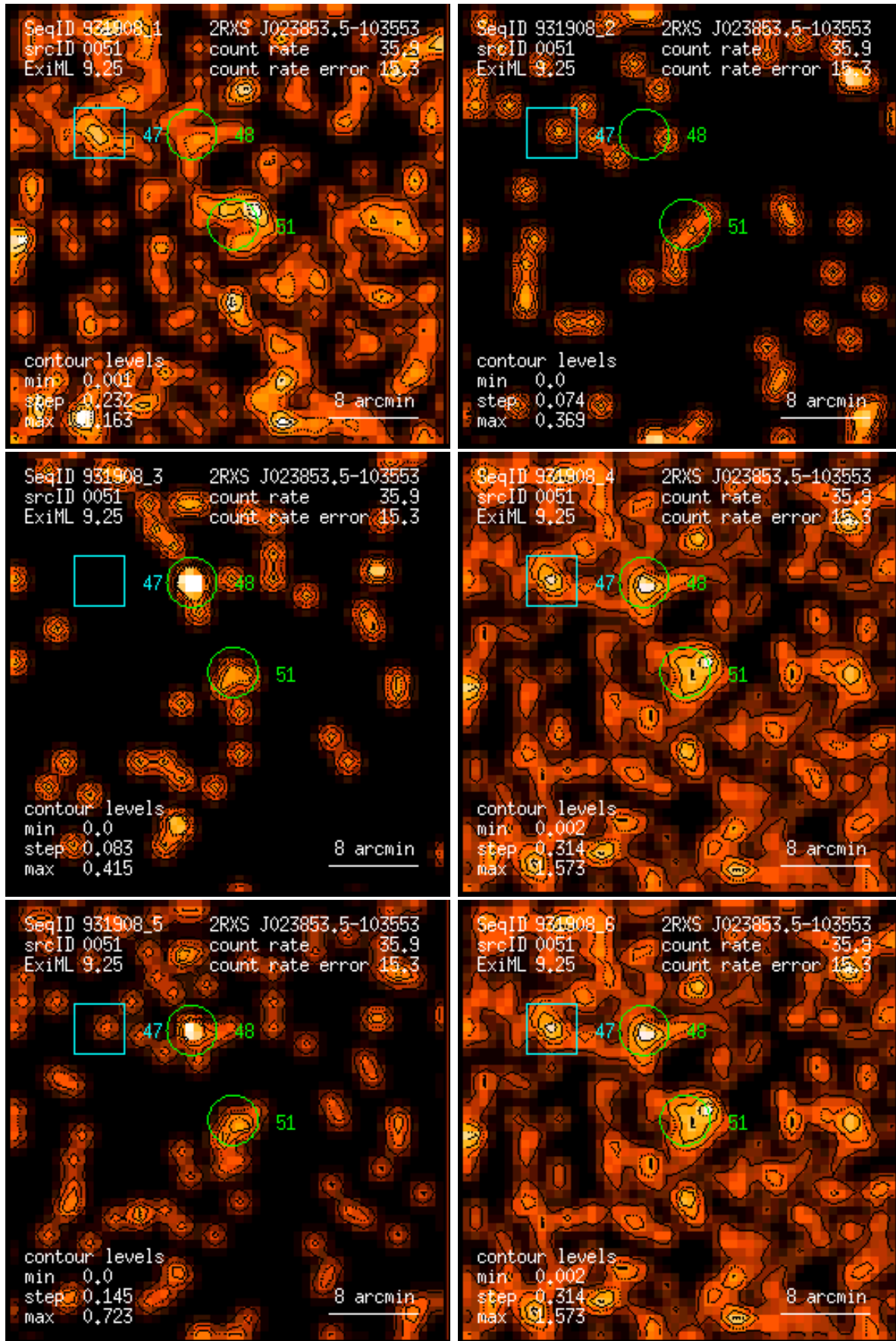
Figure 51: RASS 931908: detection 0051: band rate images, Gaussian filter: (1) PSPC channels 11 – 41, (2) 52 – 90, (3) 91 – 201, (4) 11 – 235, (5) 52 – 201, (6) 11 – 201. Broad band rates in counts/ks. Band rate contour levels in counts/ks/arcmin 2 .
