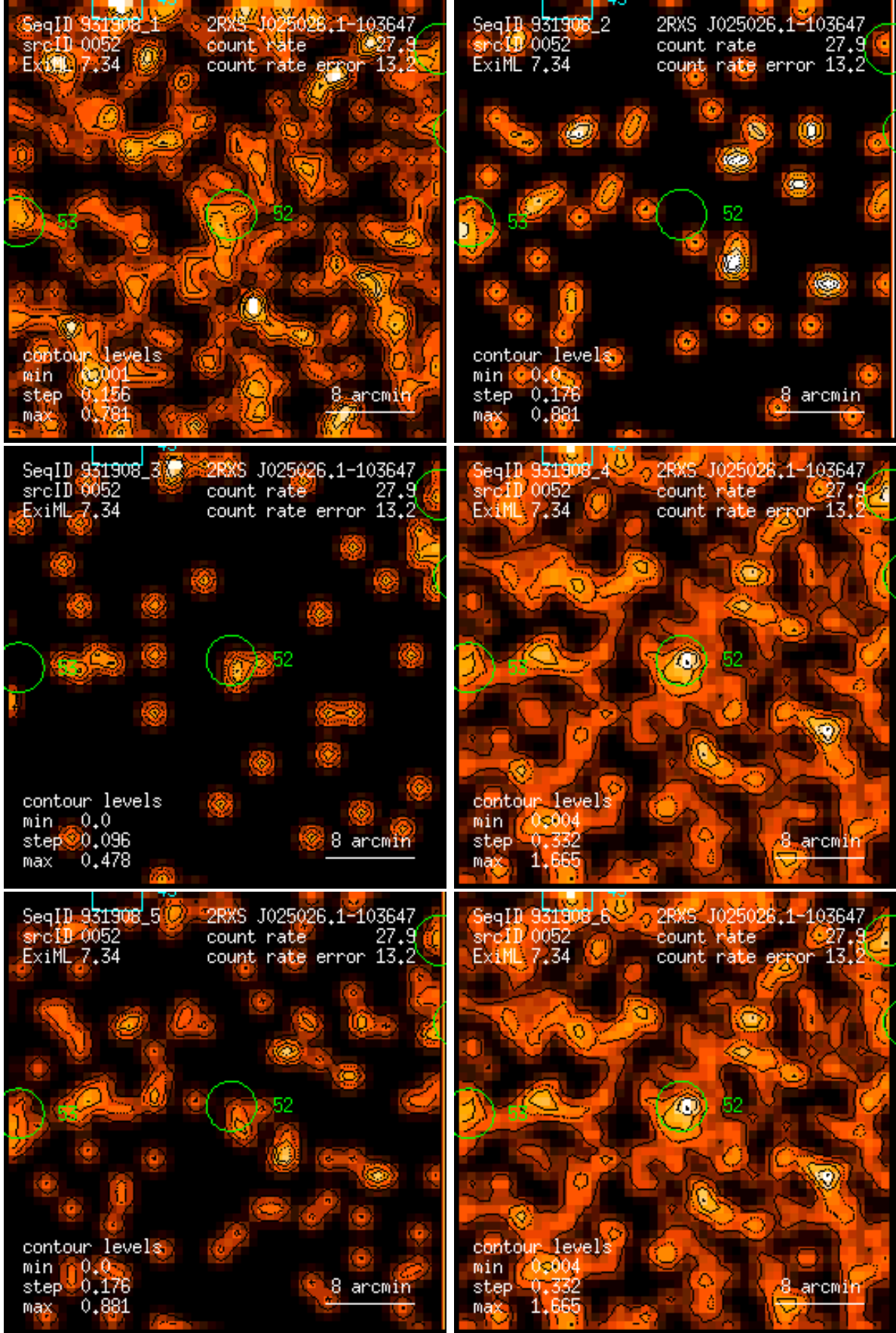
Figure 52: RASS 931908: detection 0052: band rate images, Gaussian filter: (1) PSPC channels 11 – 41, (2) 52 – 90, (3) 91 – 201, (4) 11 – 235, (5) 52 – 201, (6) 11 – 201. Broad band rates in counts/ks. Band rate contour levels in counts/ks/arcmin 2 .
