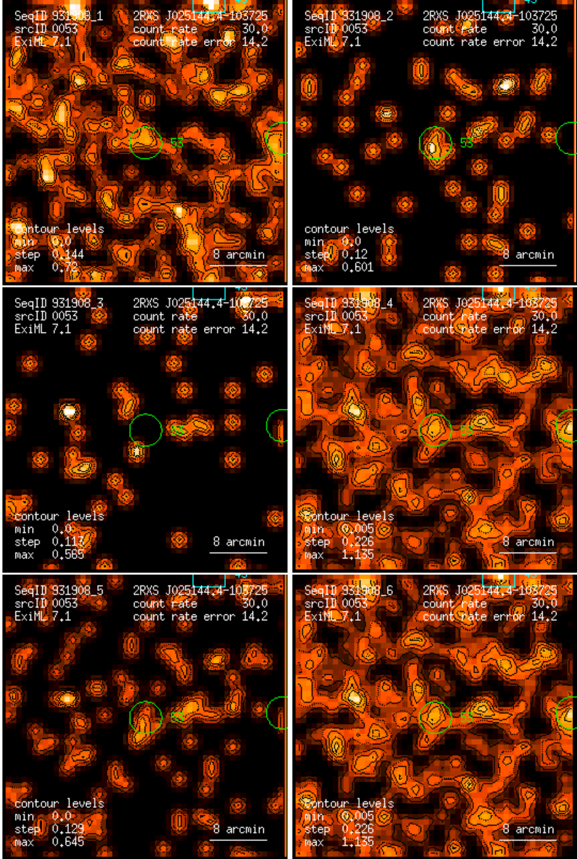
Figure 53: RASS 931908: detection 0053: band rate images, Gaussian filter: (1) PSPC channels 11 – 41, (2) 52 – 90, (3) 91 – 201, (4) 11 – 235, (5) 52 – 201, (6) 11 – 201. Broad band rates in counts/ks. Band rate contour levels in counts/ks/arcmin 2 .
