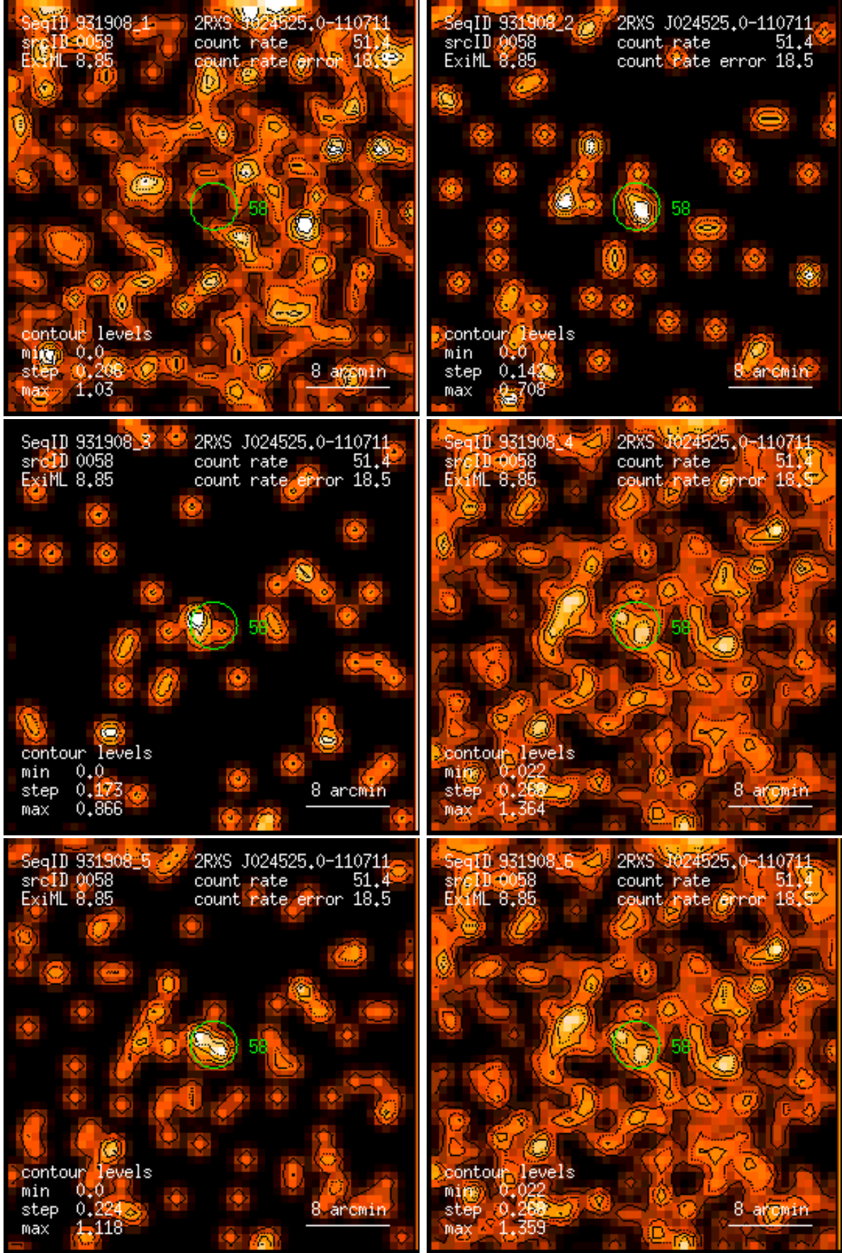
Figure 58: RASS 931908: detection 0058: band rate images, Gaussian filter: (1) PSPC channels 11 – 41, (2) 52 – 90, (3) 91 – 201, (4) 11 – 235, (5) 52 – 201, (6) 11 – 201. Broad band rates in counts/ks. Band rate contour levels in counts/ks/arcmin 2 .
