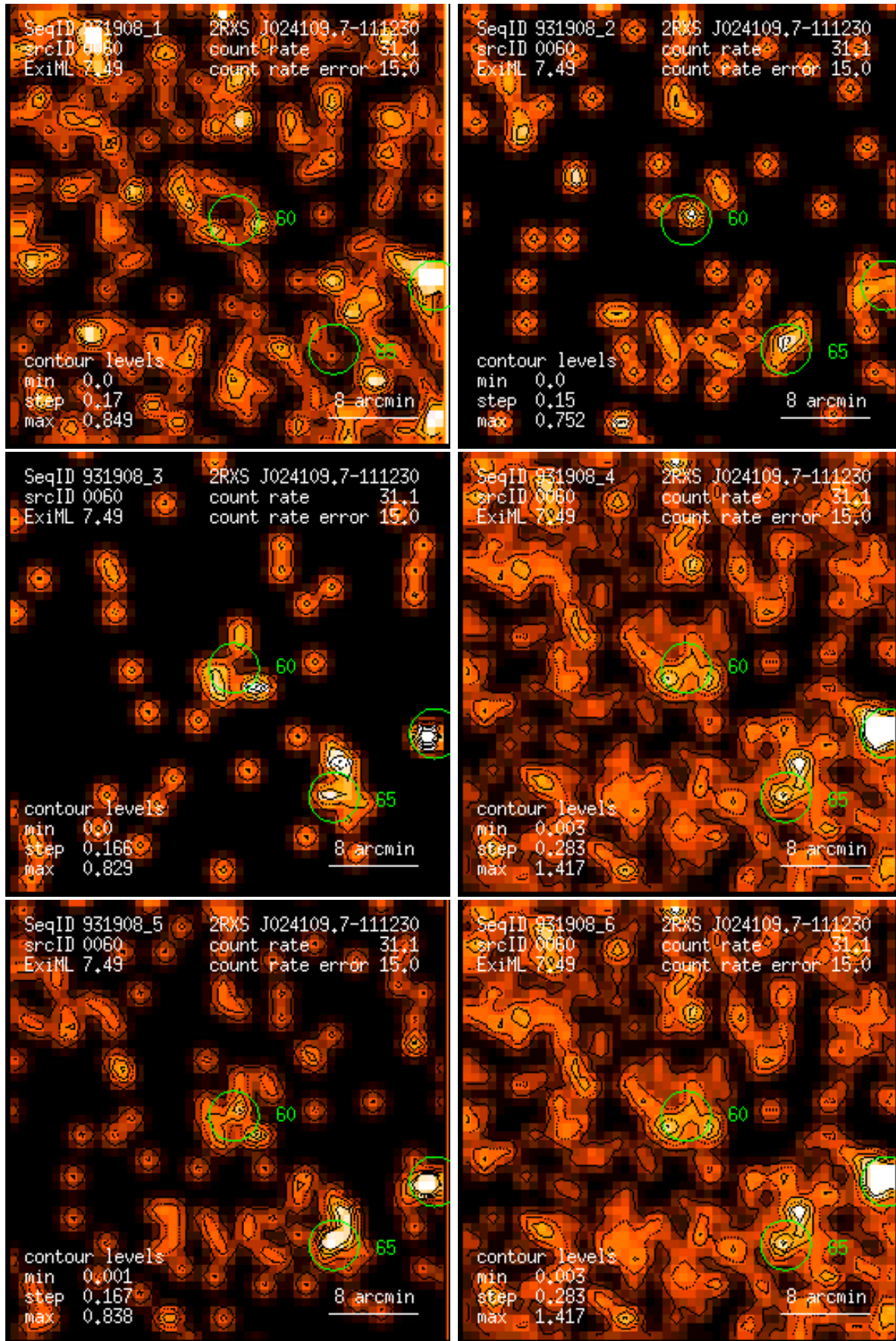
Figure 60: RASS 931908: detection 0060: band rate images, Gaussian filter: (1) PSPC channels 11 – 41, (2) 52 – 90, (3) 91 – 201, (4) 11 – 235, (5) 52 – 201, (6) 11 – 201. Broad band rates in counts/ks. Band rate contour levels in counts/ks/arcmin 2 .
