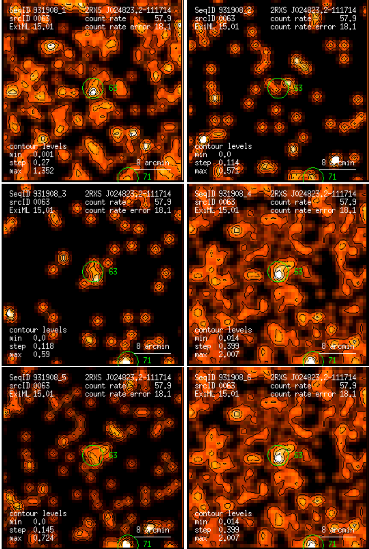
Figure 63: RASS 931908: detection 0063: band rate images, Gaussian filter: (1) PSPC channels 11 – 41, (2) 52 – 90, (3) 91 – 201, (4) 11 – 235, (5) 52 – 201, (6) 11 – 201. Broad band rates in counts/ks. Band rate contour levels in counts/ks/arcmin 2 .
