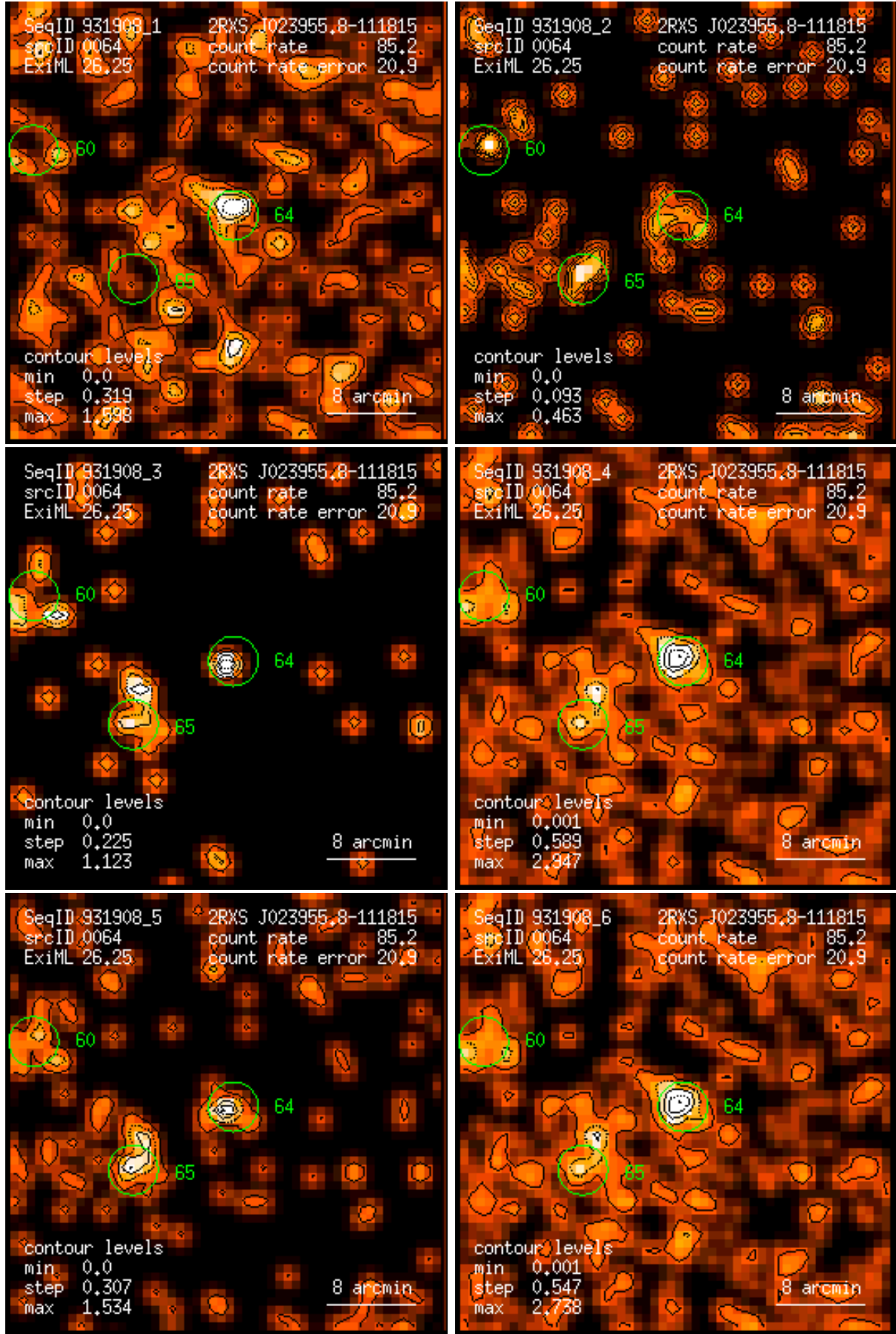
Figure 64: RASS 931908: detection 0064: band rate images, Gaussian filter: (1) PSPC channels 11 – 41, (2) 52 – 90, (3) 91 – 201, (4) 11 – 235, (5) 52 – 201, (6) 11 – 201. Broad band rates in counts/ks. Band rate contour levels in counts/ks/arcmin 2 .
