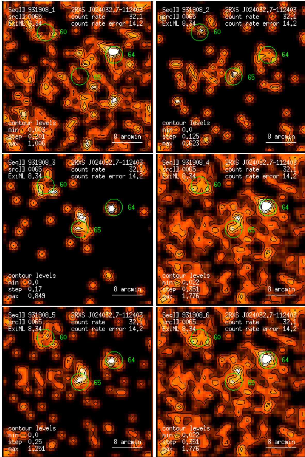
Figure 65: RASS 931908: detection 0065: band rate images, Gaussian filter: (1) PSPC channels 11 – 41, (2) 52 – 90, (3) 91 – 201, (4) 11 – 235, (5) 52 – 201, (6) 11 – 201. Broad band rates in counts/ks. Band rate contour levels in counts/ks/arcmin 2 .
