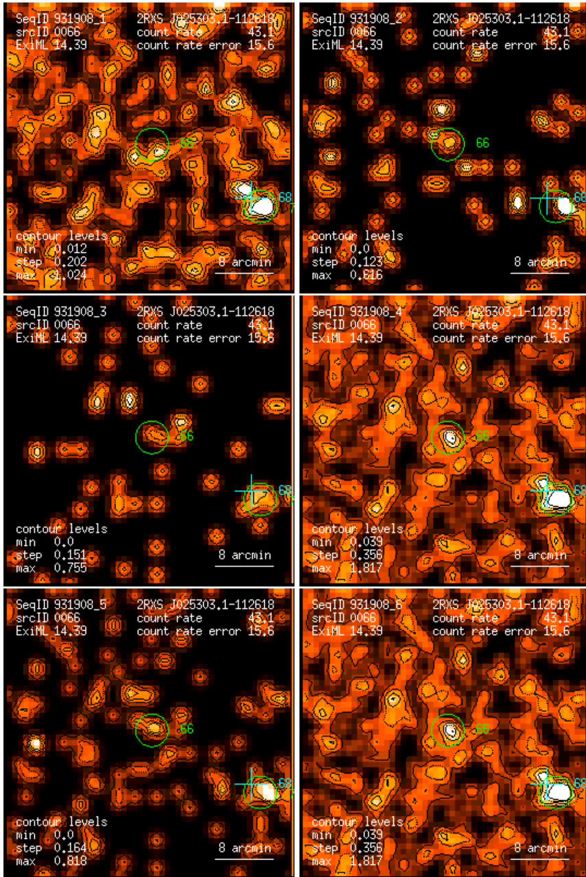
Figure 66: RASS 931908: detection 0066: band rate images, Gaussian filter: (1) PSPC channels 11 – 41, (2) 52 – 90, (3) 91 – 201, (4) 11 – 235, (5) 52 – 201, (6) 11 – 201. Broad band rates in counts/ks. Band rate contour levels in counts/ks/arcmin 2 .
