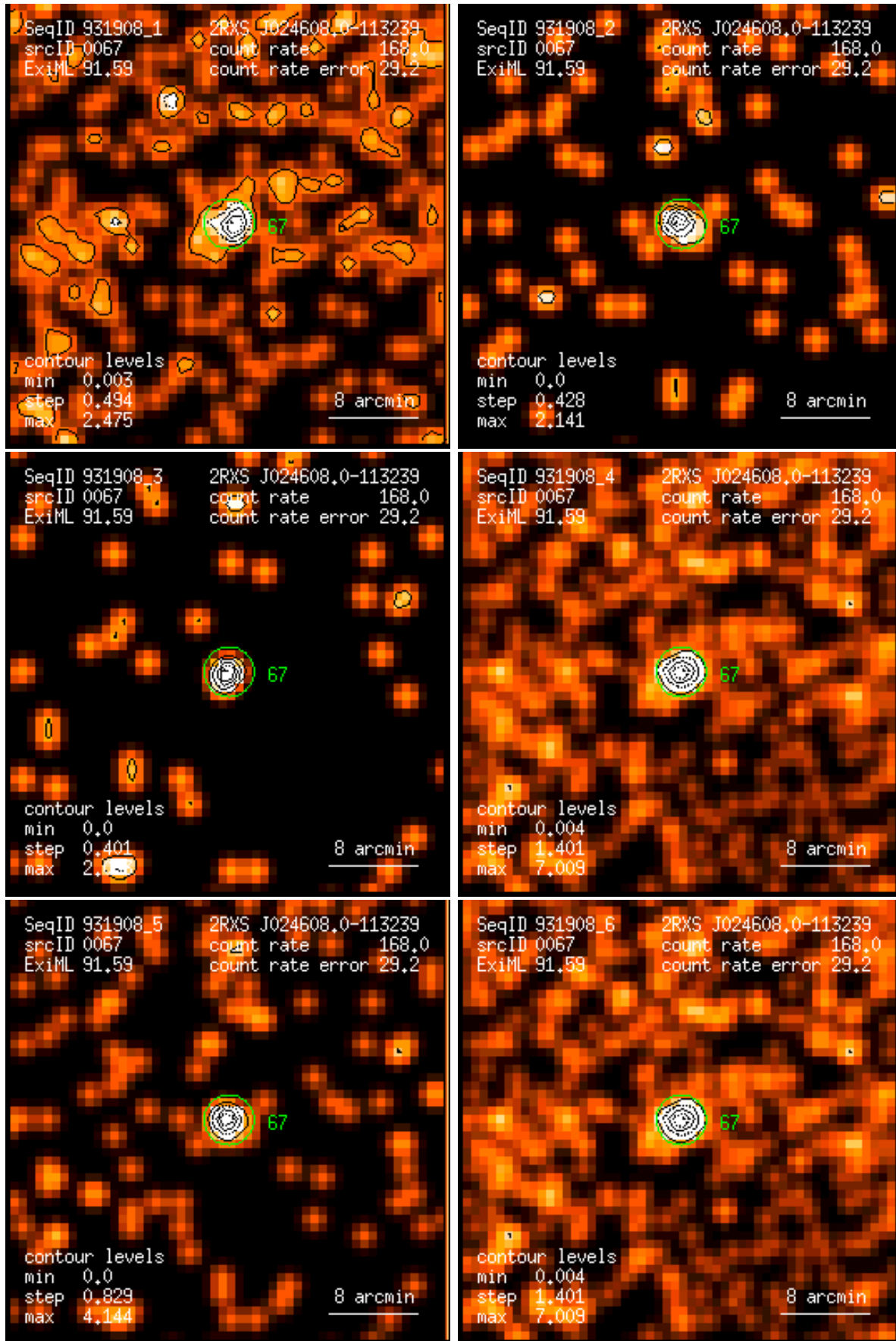
Figure 67: RASS 931908: detection 0067: band rate images, Gaussian filter: (1) PSPC channels 11 – 41, (2) 52 – 90, (3) 91 – 201, (4) 11 – 235, (5) 52 – 201, (6) 11 – 201. Broad band rates in counts/ks. Band rate contour levels in counts/ks/arcmin 2 .
