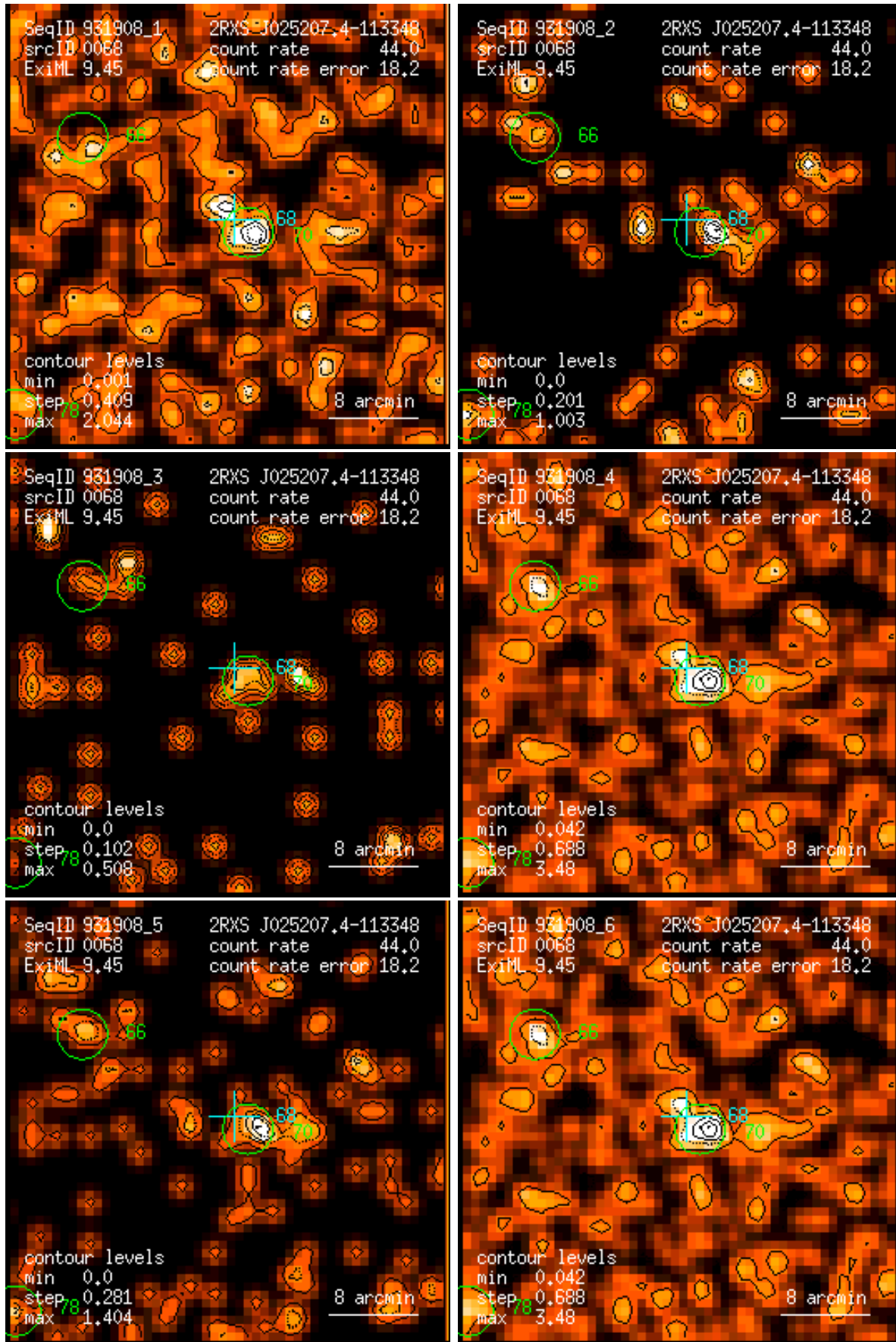
Figure 68: RASS 931908: detection 0068: band rate images, Gaussian filter: (1) PSPC channels 11 – 41, (2) 52 – 90, (3) 91 – 201, (4) 11 – 235, (5) 52 – 201, (6) 11 – 201. Broad band rates in counts/ks. Band rate contour levels in counts/ks/arcmin 2 .
