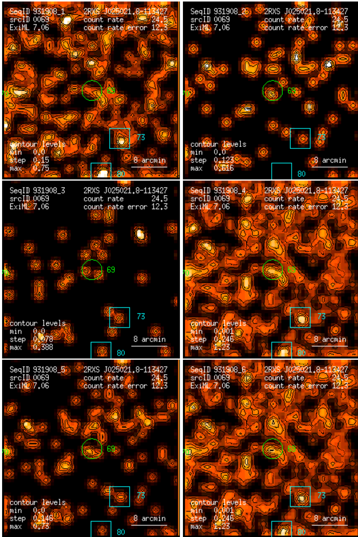
Figure 69: RASS 931908: detection 0069: band rate images, Gaussian filter: (1) PSPC channels 11 – 41, (2) 52 – 90, (3) 91 – 201, (4) 11 – 235, (5) 52 – 201, (6) 11 – 201. Broad band rates in counts/ks. Band rate contour levels in counts/ks/arcmin 2 .
