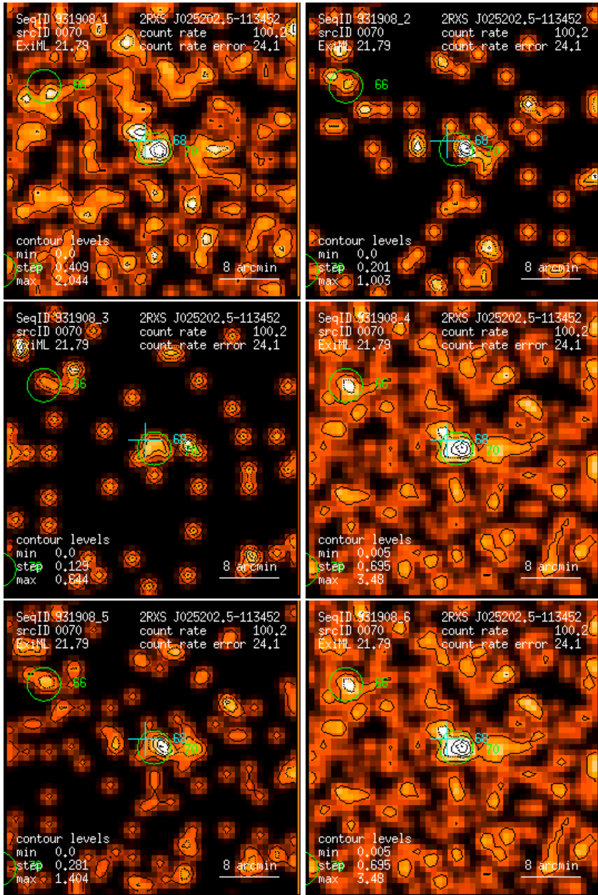
Figure 70: RASS 931908: detection 0070: band rate images, Gaussian filter: (1) PSPC channels 11 – 41, (2) 52 – 90, (3) 91 – 201, (4) 11 – 235, (5) 52 – 201, (6) 11 – 201. Broad band rates in counts/ks. Band rate contour levels in counts/ks/arcmin 2 .
