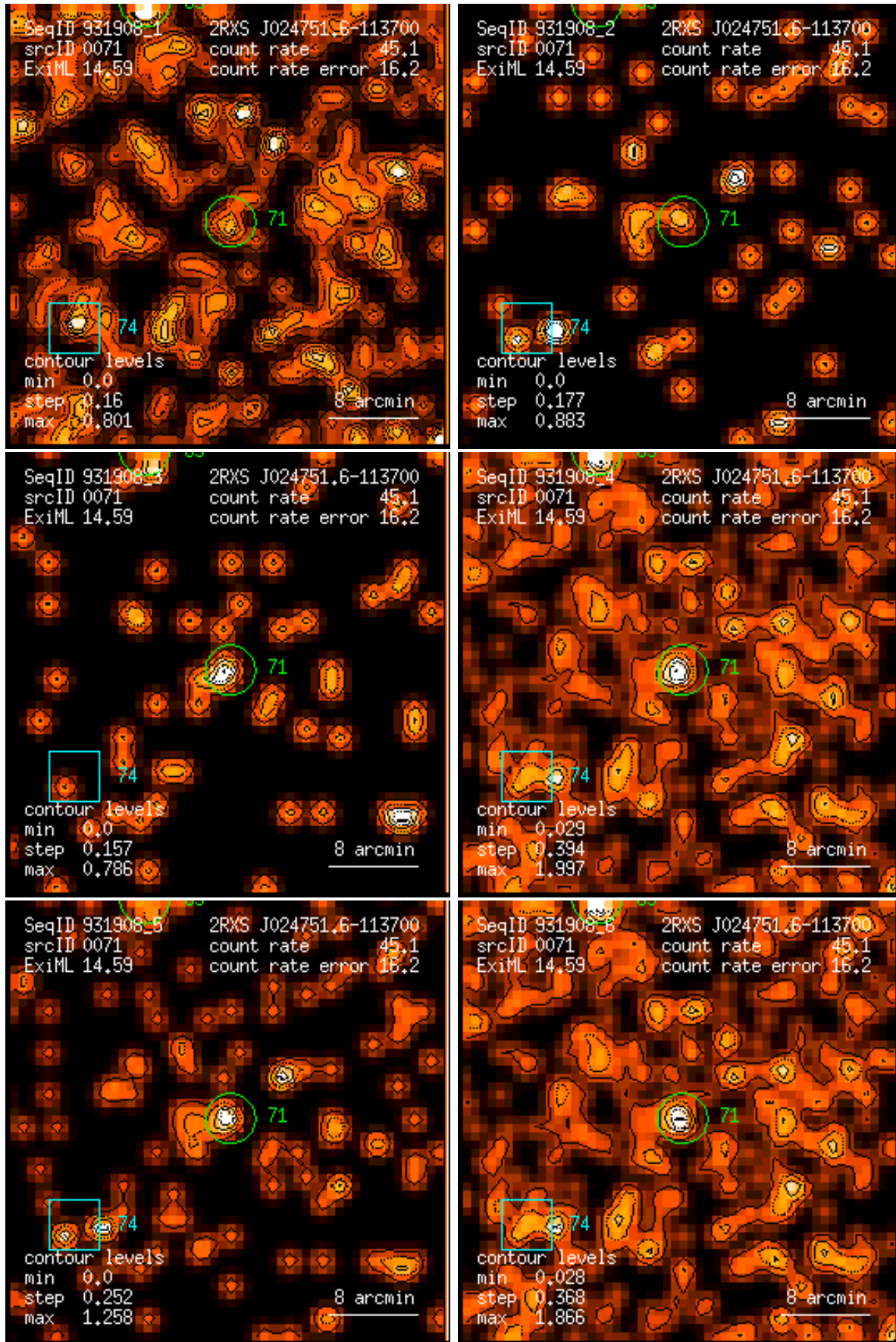
Figure 71: RASS 931908: detection 0071: band rate images, Gaussian filter: (1) PSPC channels 11 – 41, (2) 52 – 90, (3) 91 – 201, (4) 11 – 235, (5) 52 – 201, (6) 11 – 201. Broad band rates in counts/ks. Band rate contour levels in counts/ks/arcmin 2 .
