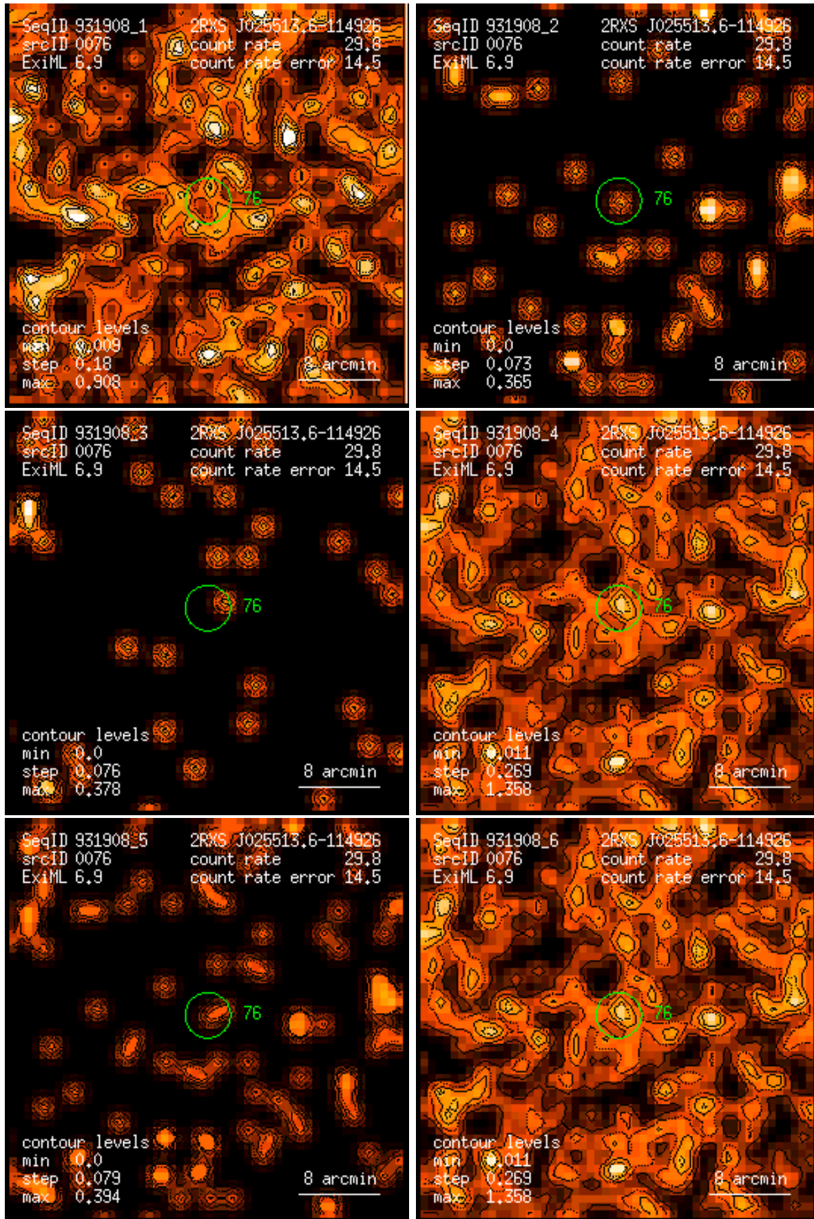
Figure 76: RASS 931908: detection 0076: band rate images, Gaussian filter: (1) PSPC channels 11 – 41, (2) 52 – 90, (3) 91 – 201, (4) 11 – 235, (5) 52 – 201, (6) 11 – 201. Broad band rates in counts/ks. Band rate contour levels in counts/ks/arcmin 2 .
