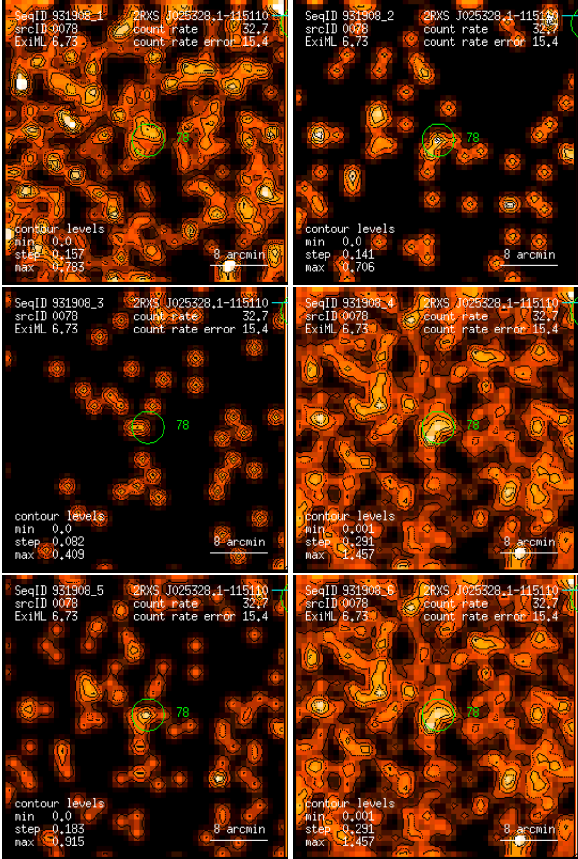
Figure 78: RASS 931908: detection 0078: band rate images, Gaussian filter: (1) PSPC channels 11 – 41, (2) 52 – 90, (3) 91 – 201, (4) 11 – 235, (5) 52 – 201, (6) 11 – 201. Broad band rates in counts/ks. Band rate contour levels in counts/ks/arcmin 2 .
