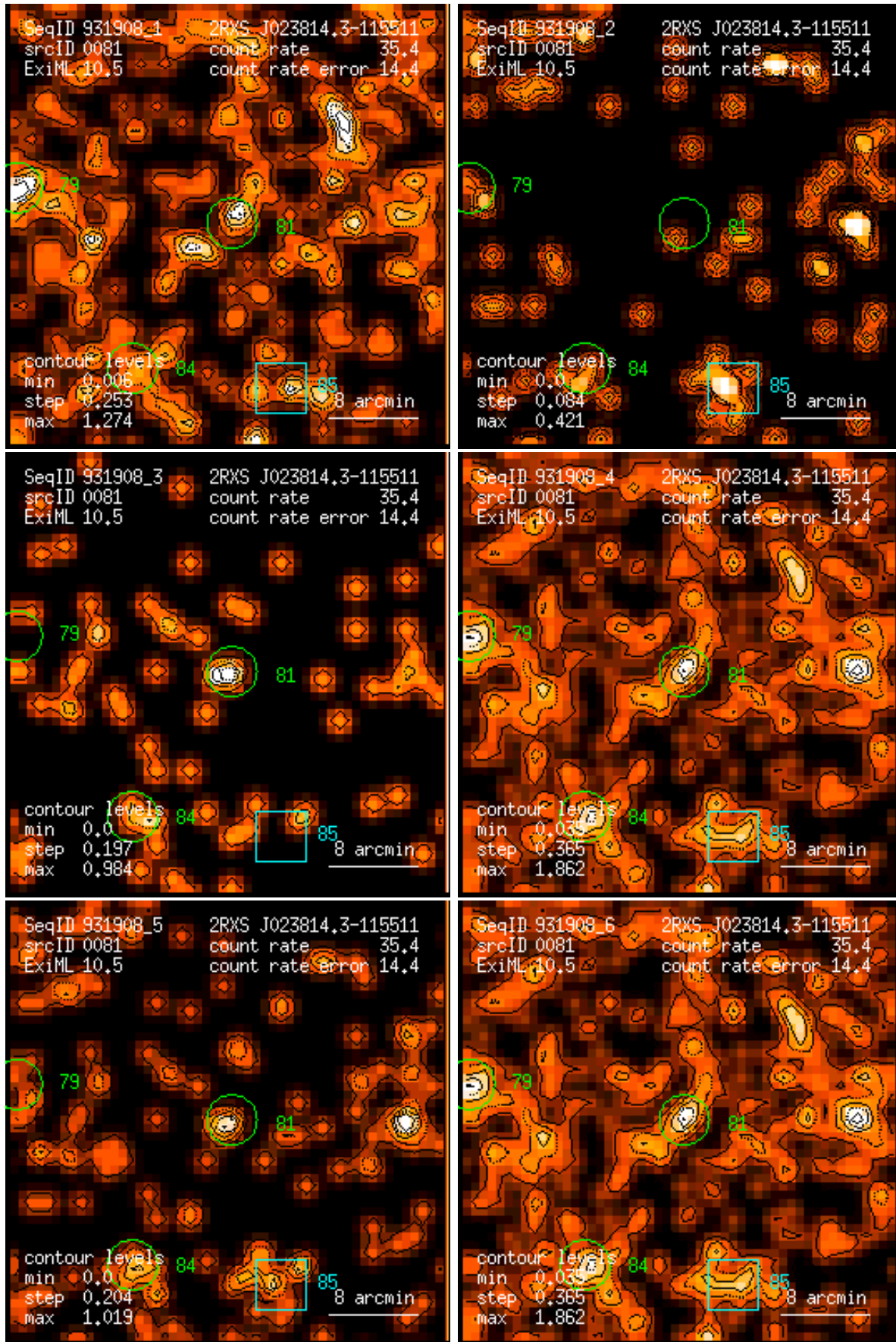
Figure 81: RASS 931908: detection 0081: band rate images, Gaussian filter: (1) PSPC channels 11 – 41, (2) 52 – 90, (3) 91 – 201, (4) 11 – 235, (5) 52 – 201, (6) 11 – 201. Broad band rates in counts/ks. Band rate contour levels in counts/ks/arcmin 2 .
