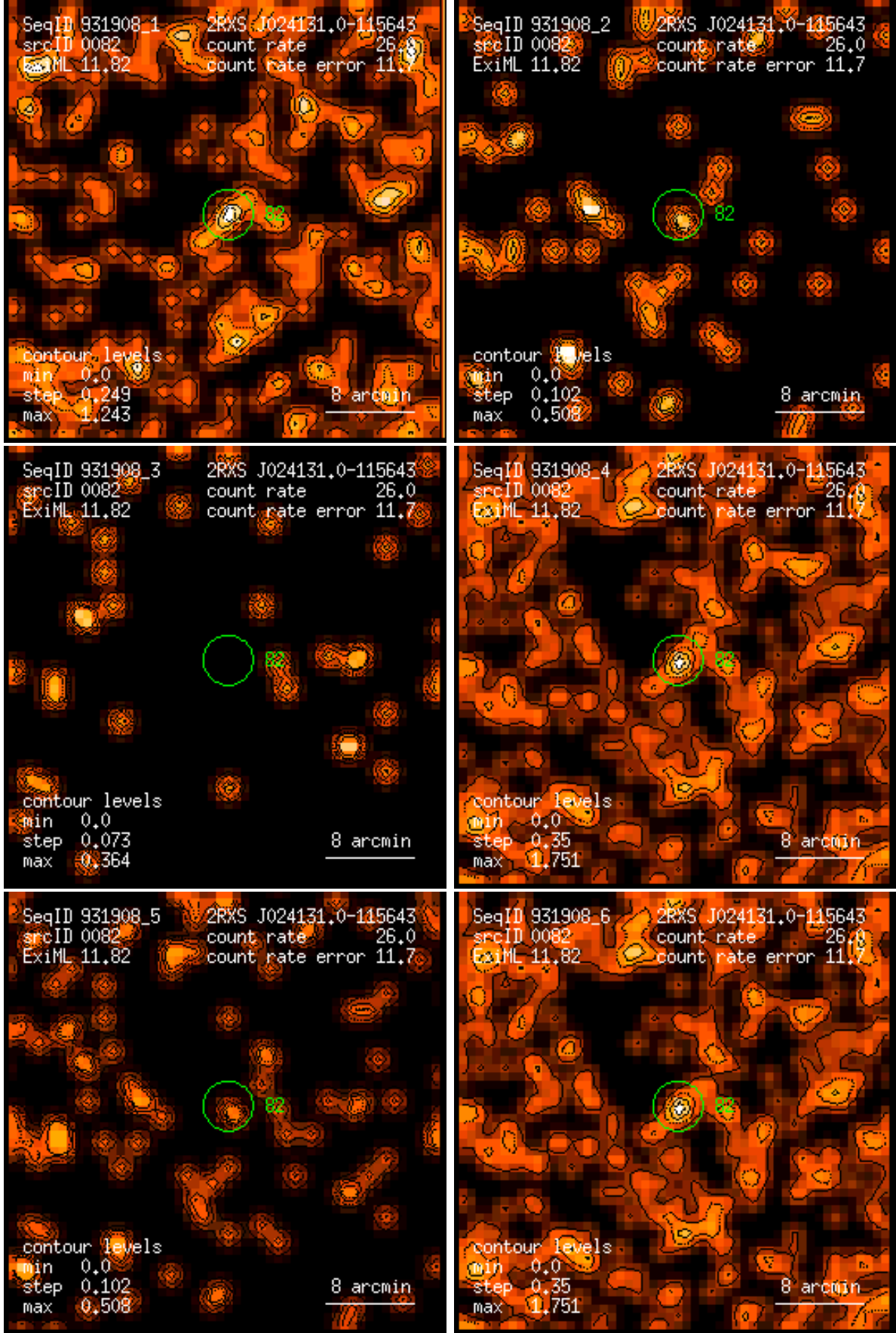
Figure 82: RASS 931908: detection 0082: band rate images, Gaussian filter: (1) PSPC channels 11 – 41, (2) 52 – 90, (3) 91 – 201, (4) 11 – 235, (5) 52 – 201, (6) 11 – 201. Broad band rates in counts/ks. Band rate contour levels in counts/ks/arcmin 2 .
