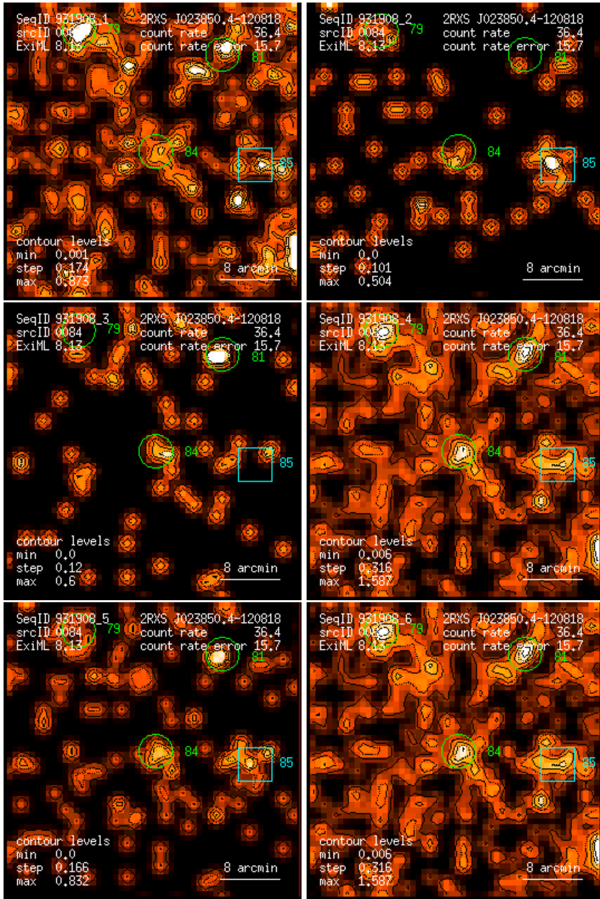
Figure 84: RASS 931908: detection 0084: band rate images, Gaussian filter: (1) PSPC channels 11 – 41, (2) 52 – 90, (3) 91 – 201, (4) 11 – 235, (5) 52 – 201, (6) 11 – 201. Broad band rates in counts/ks. Band rate contour levels in counts/ks/arcmin 2 .
