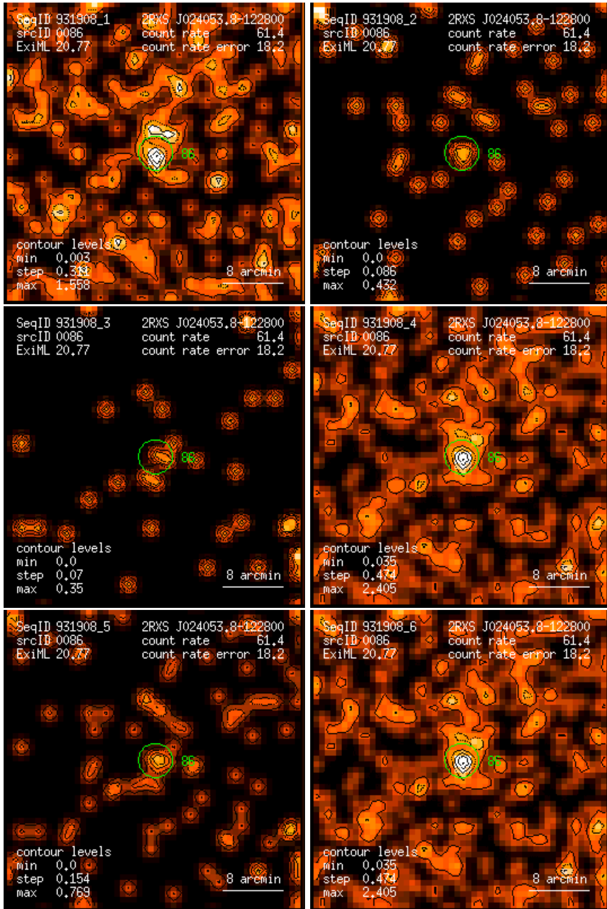
Figure 86: RASS 931908: detection 0086: band rate images, Gaussian filter: (1) PSPC channels 11 – 41, (2) 52 – 90, (3) 91 – 201, (4) 11 – 235, (5) 52 – 201, (6) 11 – 201. Broad band rates in counts/ks. Band rate contour levels in counts/ks/arcmin 2 .
