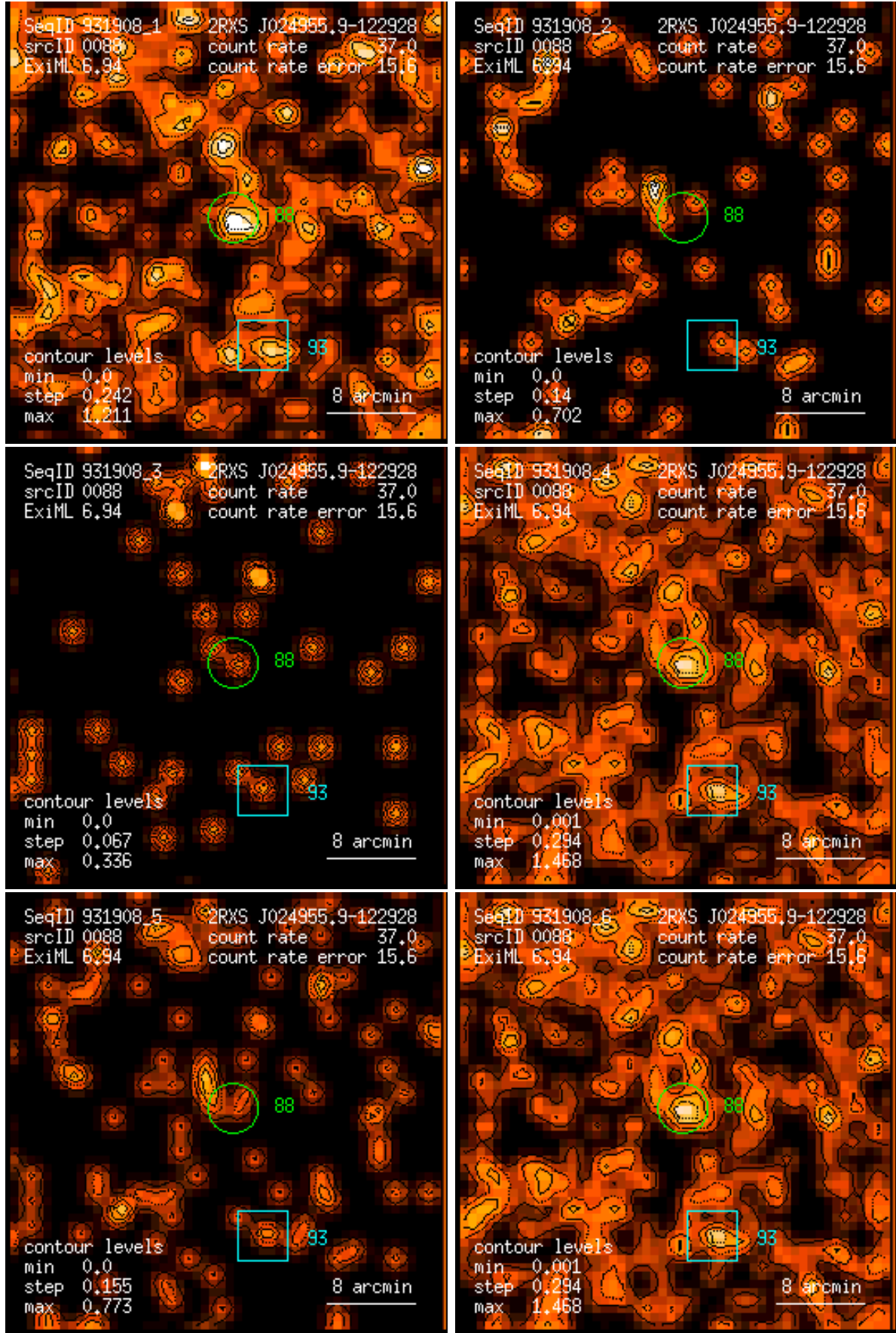
Figure 88: RASS 931908: detection 0088: band rate images, Gaussian filter: (1) PSPC channels 11 – 41, (2) 52 – 90, (3) 91 – 201, (4) 11 – 235, (5) 52 – 201, (6) 11 – 201. Broad band rates in counts/ks. Band rate contour levels in counts/ks/arcmin 2 .
