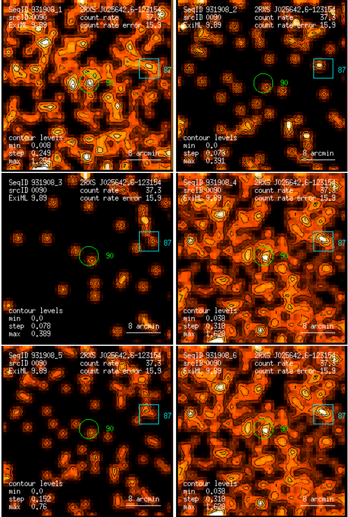
Figure 90: RASS 931908: detection 0090: band rate images, Gaussian filter: (1) PSPC channels 11 – 41, (2) 52 – 90, (3) 91 – 201, (4) 11 – 235, (5) 52 – 201, (6) 11 – 201. Broad band rates in counts/ks. Band rate contour levels in counts/ks/arcmin 2 .
