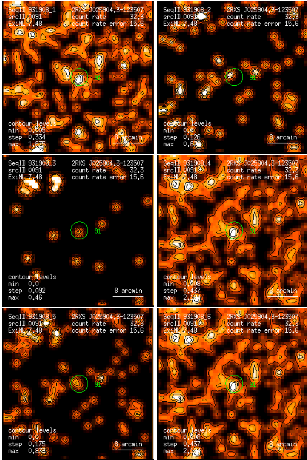
Figure 91: RASS 931908: detection 0091: band rate images, Gaussian filter: (1) PSPC channels 11 – 41, (2) 52 – 90, (3) 91 – 201, (4) 11 – 235, (5) 52 – 201, (6) 11 – 201. Broad band rates in counts/ks. Band rate contour levels in counts/ks/arcmin 2 .
