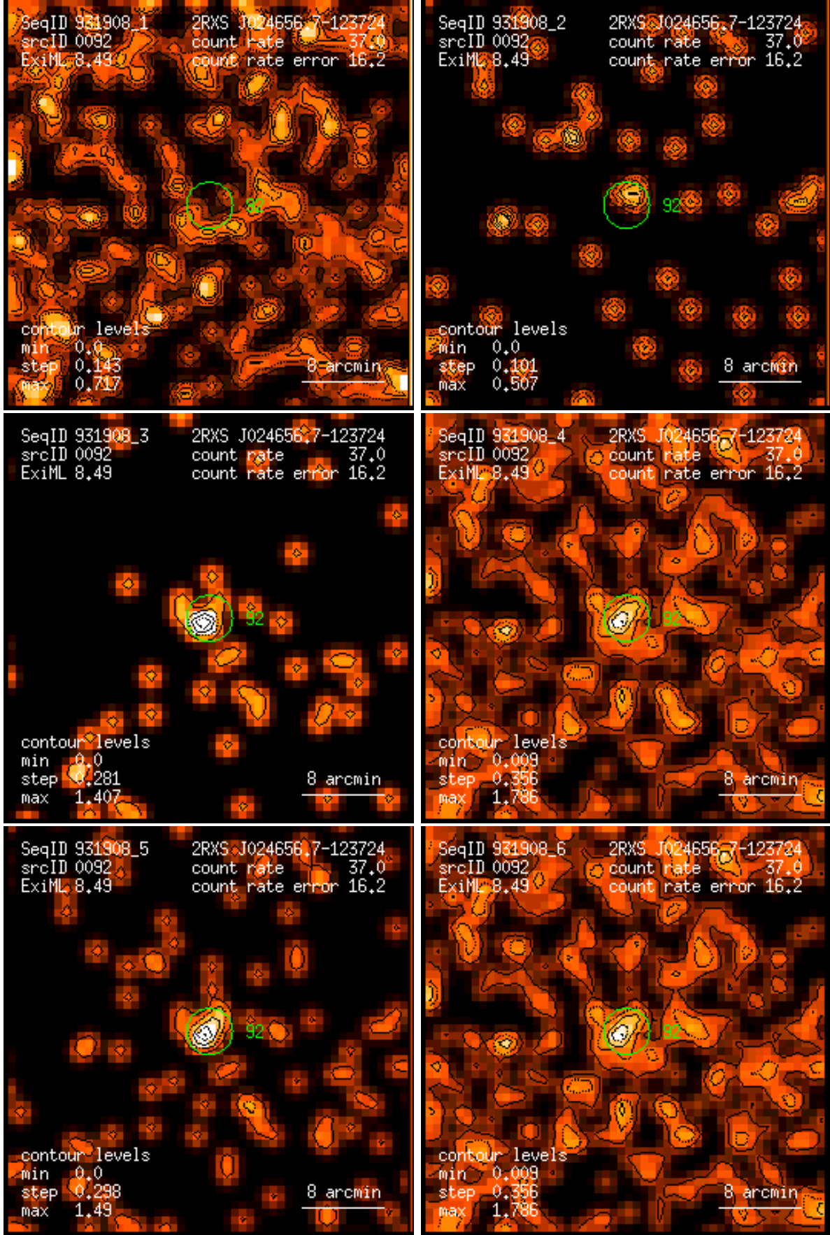
Figure 92: RASS 931908: detection 0092: band rate images, Gaussian filter: (1) PSPC channels 11 – 41, (2) 52 – 90, (3) 91 – 201, (4) 11 – 235, (5) 52 – 201, (6) 11 – 201. Broad band rates in counts/ks. Band rate contour levels in counts/ks/arcmin 2 .
