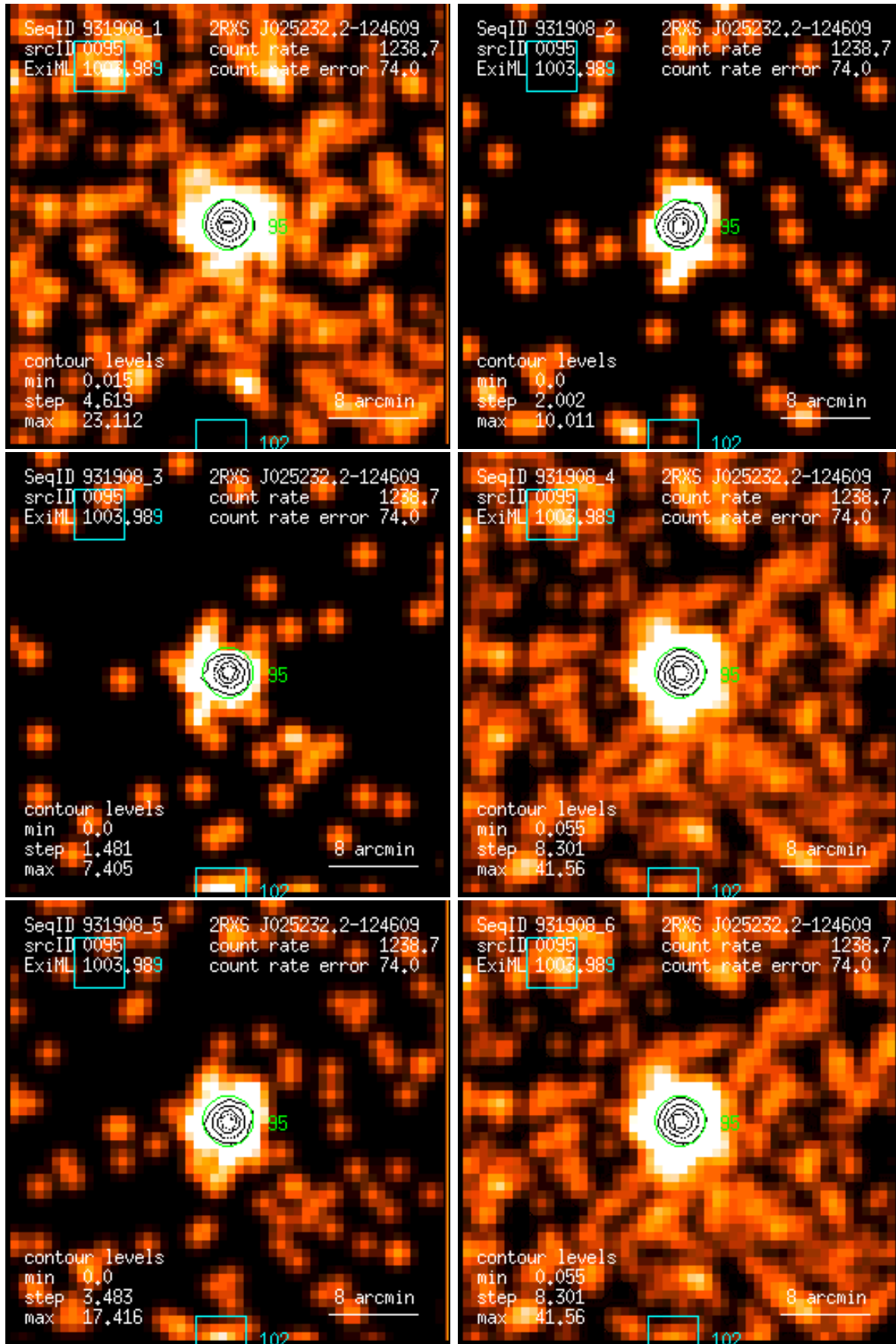
Figure 95: RASS 931908: detection 0095: band rate images, Gaussian filter: (1) PSPC channels 11 – 41, (2) 52 – 90, (3) 91 – 201, (4) 11 – 235, (5) 52 – 201, (6) 11 – 201. Broad band rates in counts/ks. Band rate contour levels in counts/ks/arcmin 2 .
