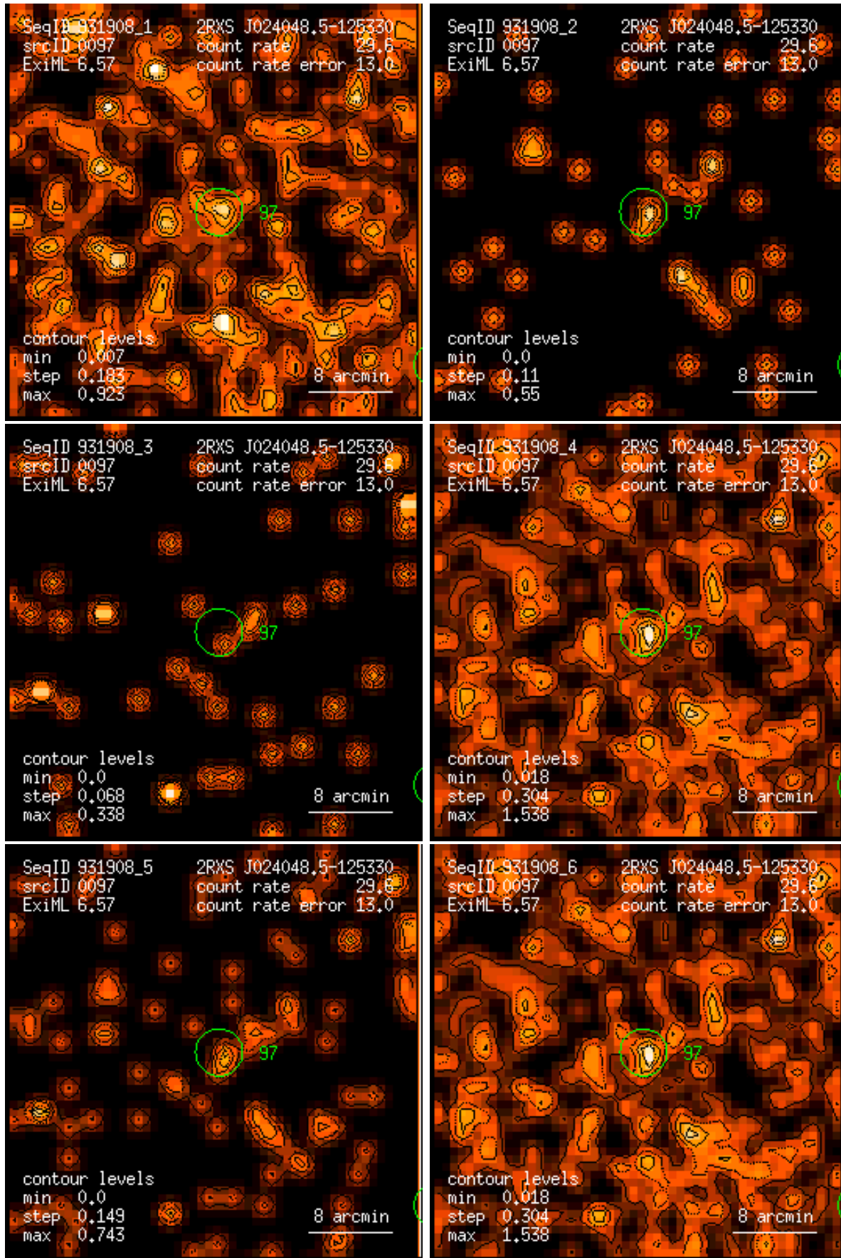
Figure 97: RASS 931908: detection 0097: band rate images, Gaussian filter: (1) PSPC channels 11 – 41, (2) 52 – 90, (3) 91 – 201, (4) 11 – 235, (5) 52 – 201, (6) 11 – 201. Broad band rates in counts/ks. Band rate contour levels in counts/ks/arcmin 2 .
