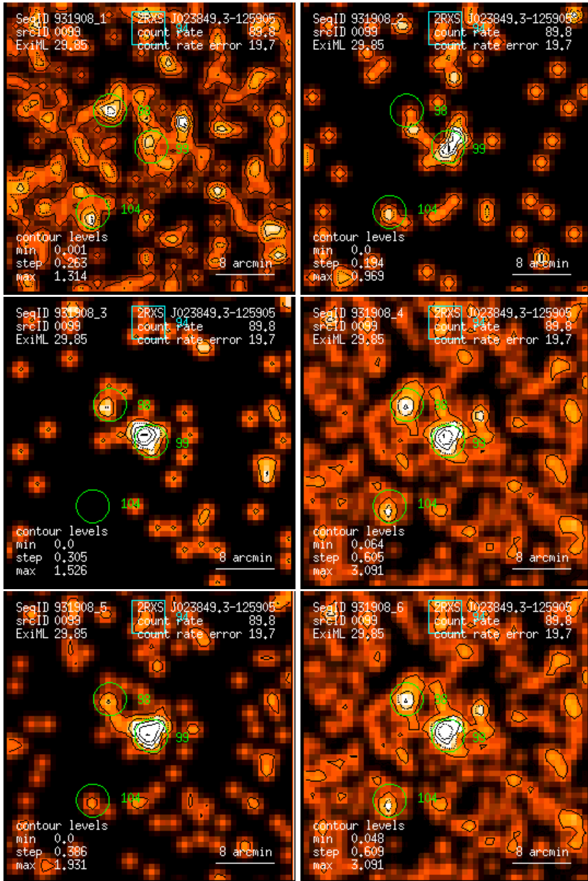
Figure 99: RASS 931908: detection 0099: band rate images, Gaussian filter: (1) PSPC channels 11 – 41, (2) 52 – 90, (3) 91 – 201, (4) 11 – 235, (5) 52 – 201, (6) 11 – 201. Broad band rates in counts/ks. Band rate contour levels in counts/ks/arcmin 2 .
