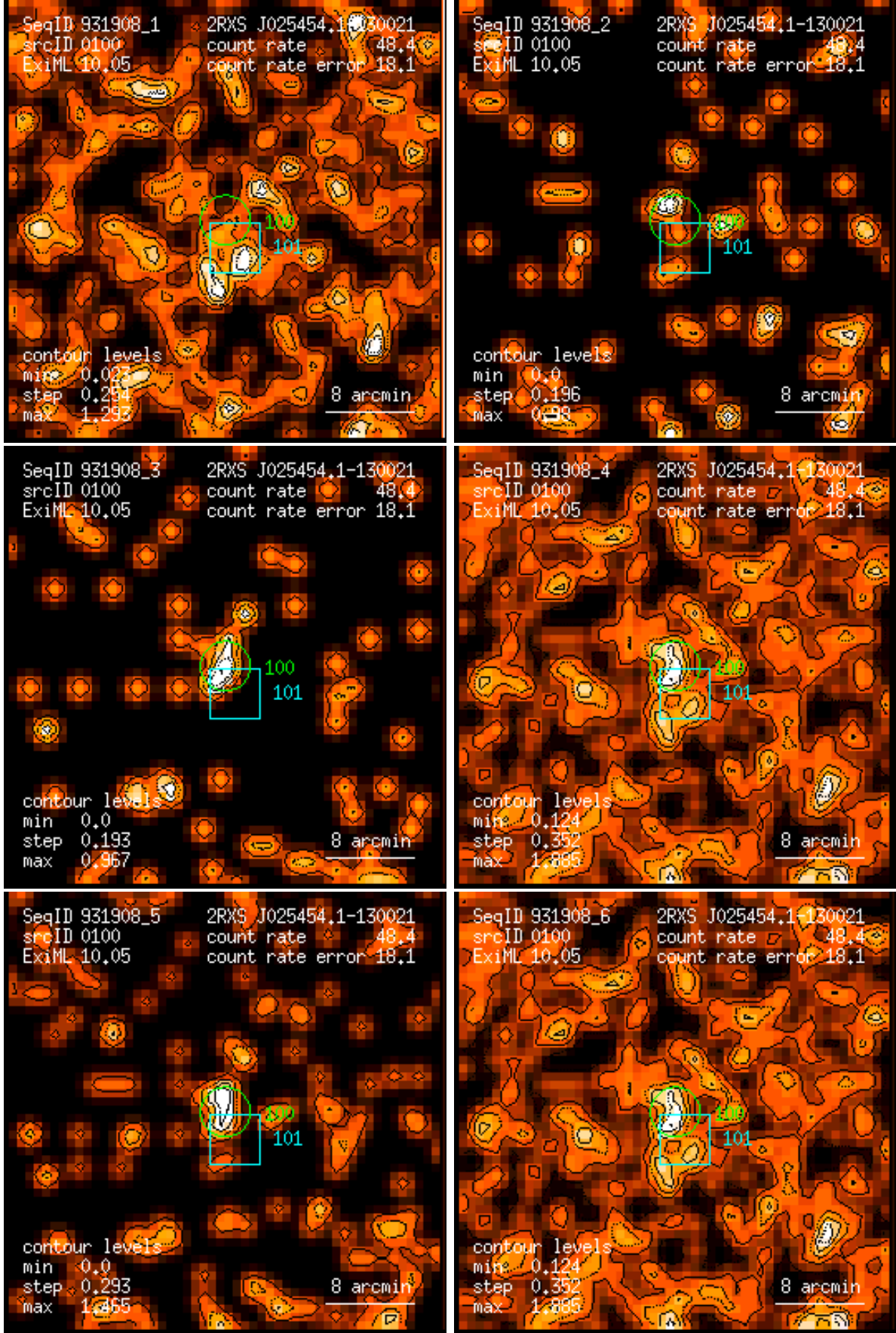
Figure 100: RASS 931908: detection 0100: band rate images, Gaussian filter: (1) PSPC channels 11 – 41, (2) 52 – 90, (3) 91 – 201, (4) 11 – 235, (5) 52 – 201, (6) 11 – 201. Broad band rates in counts/ks. Band rate contour levels in counts/ks/arcmin 2 .
