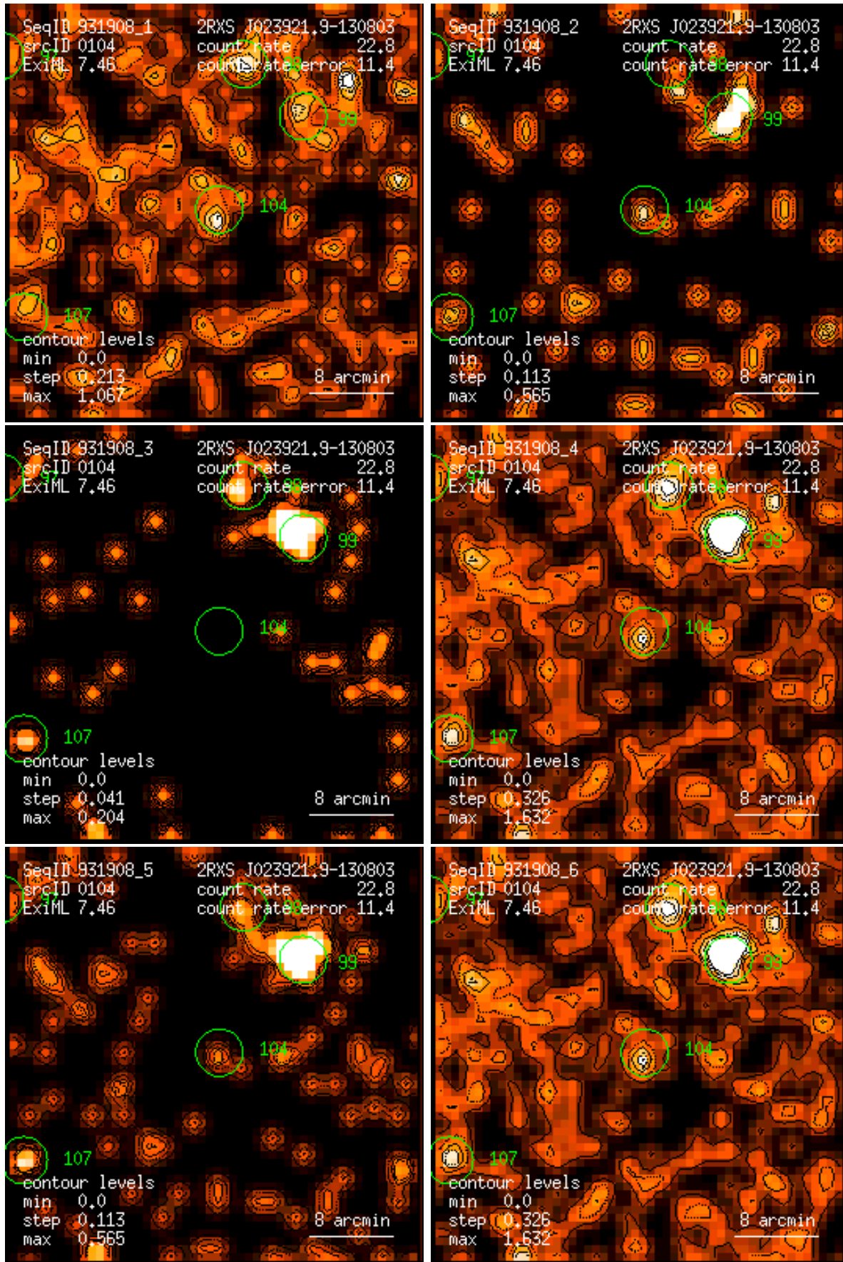
Figure 104: RASS 931908: detection 0104: band rate images, Gaussian filter: (1) PSPC channels 11 – 41, (2) 52 – 90, (3) 91 – 201, (4) 11 – 235, (5) 52 – 201, (6) 11 – 201. Broad band rates in counts/ks. Band rate contour levels in counts/ks/arcmin 2 .
