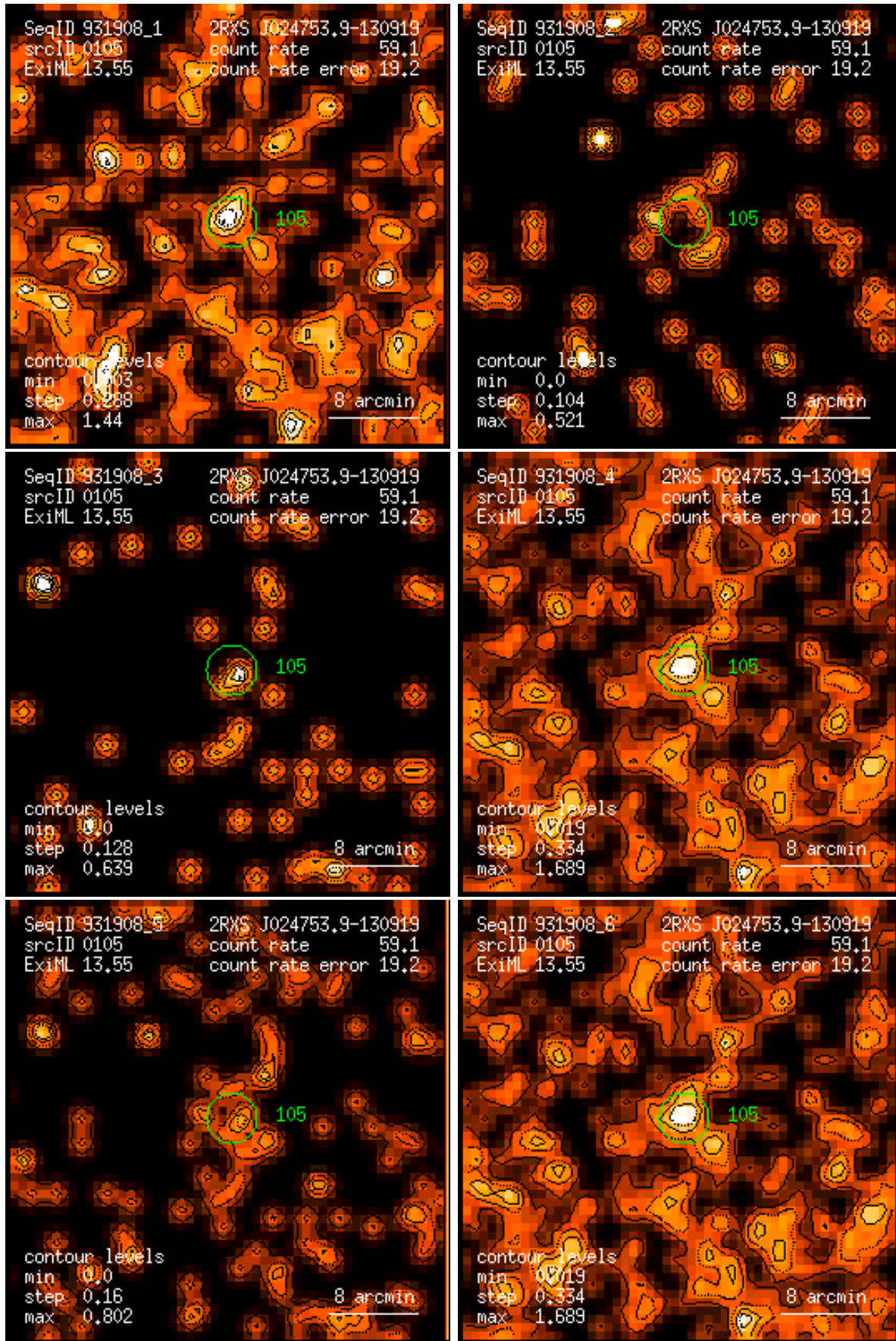
Figure 105: RASS 931908: detection 0105: band rate images, Gaussian filter: (1) PSPC channels 11 – 41, (2) 52 – 90, (3) 91 – 201, (4) 11 – 235, (5) 52 – 201, (6) 11 – 201. Broad band rates in counts/ks. Band rate contour levels in counts/ks/arcmin 2 .
