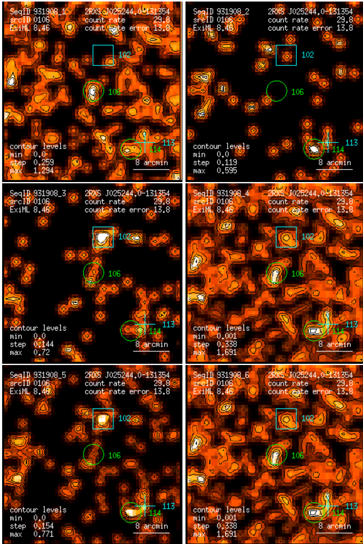
Figure 106: RASS 931908: detection 0106: band rate images, Gaussian filter: (1) PSPC channels 11 – 41, (2) 52 – 90, (3) 91 – 201, (4) 11 – 235, (5) 52 – 201, (6) 11 – 201. Broad band rates in counts/ks. Band rate contour levels in counts/ks/arcmin 2 .
